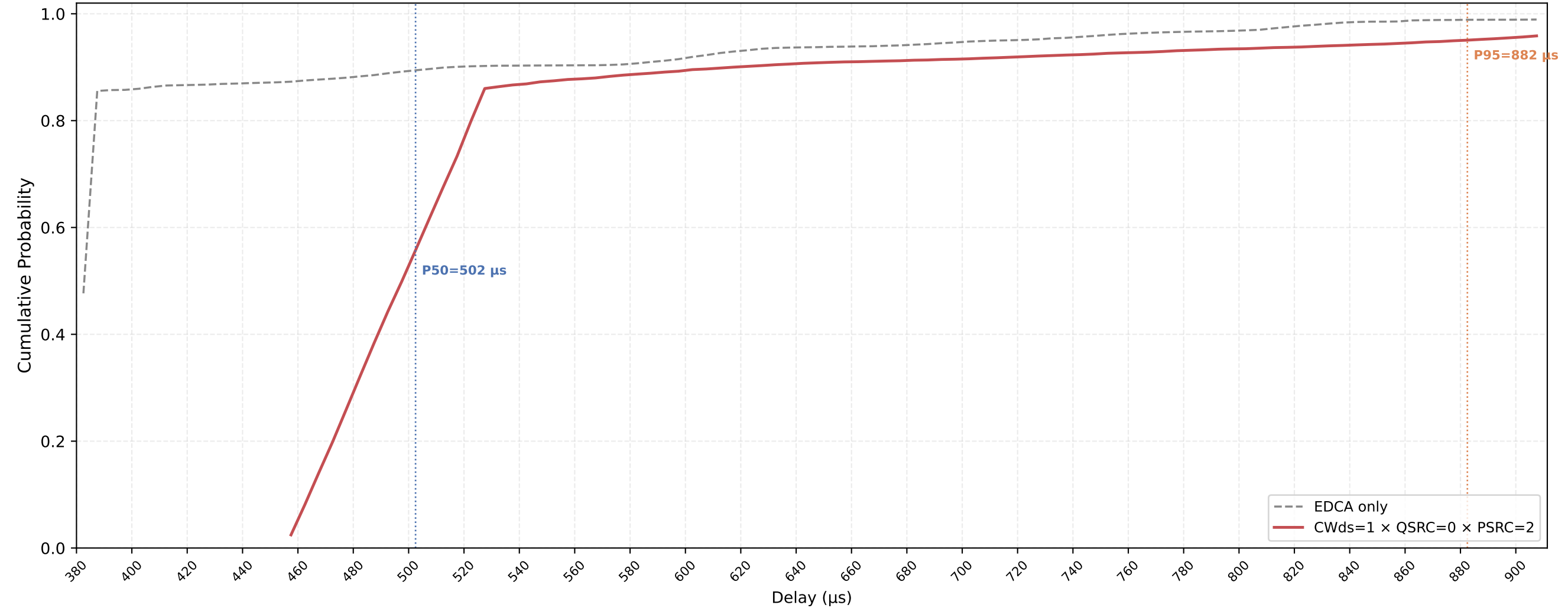
P-EDCA STA VO Delay CDF — CWds=1 × QSRC=0 × PSRC=2 nSta=30, nPedca=15, 0.1Mbps, avg of 10 runs
