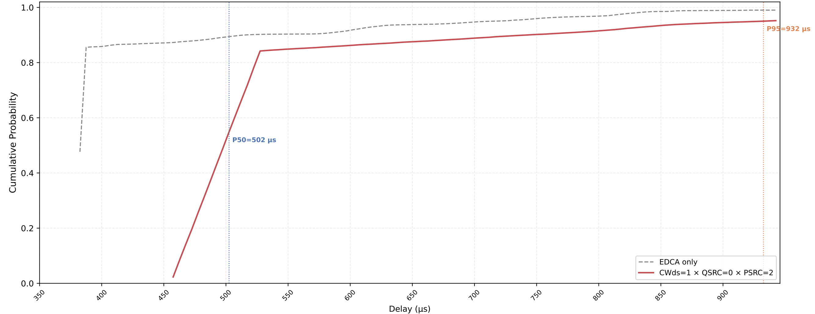
P-EDCA STA VO Delay CDF — CWds=1 × QSRC=0 × PSRC=2 nSta=30, nPedca=30, 0.1Mbps, avg of 10 runs
