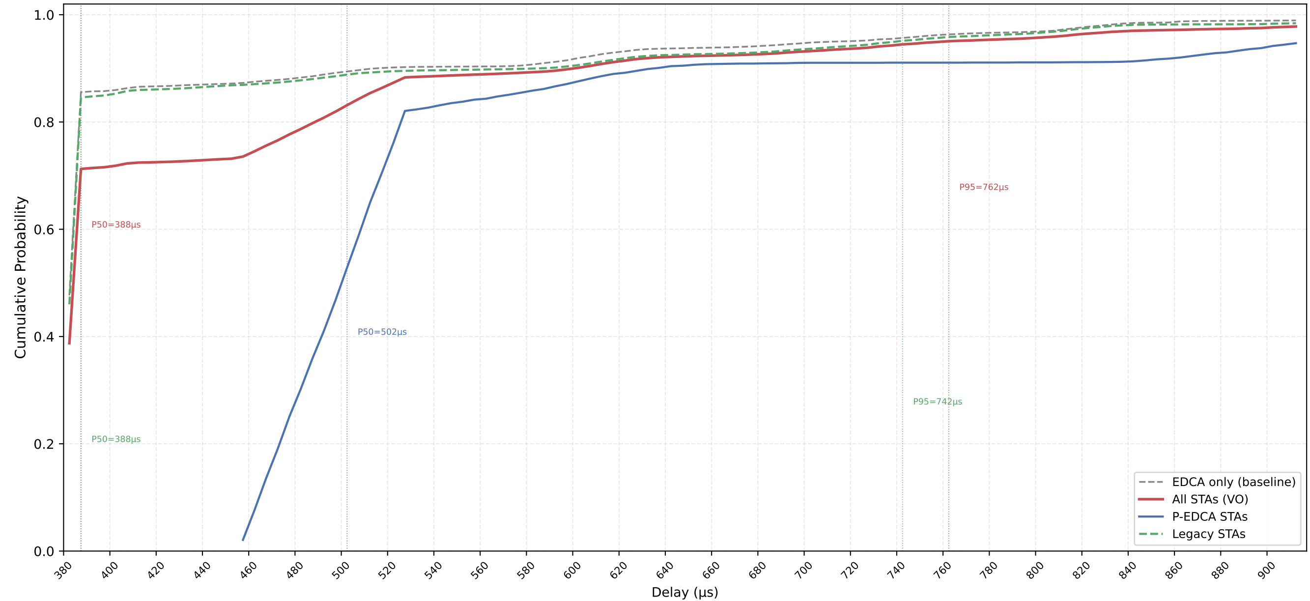
VO Delay CDF — P-EDCA / Legacy / All | CWds=1 × QSRC=0 × PSRC=3 nSta=30, nPedca=5/30, 0.1Mbps, avg of 10 runs
