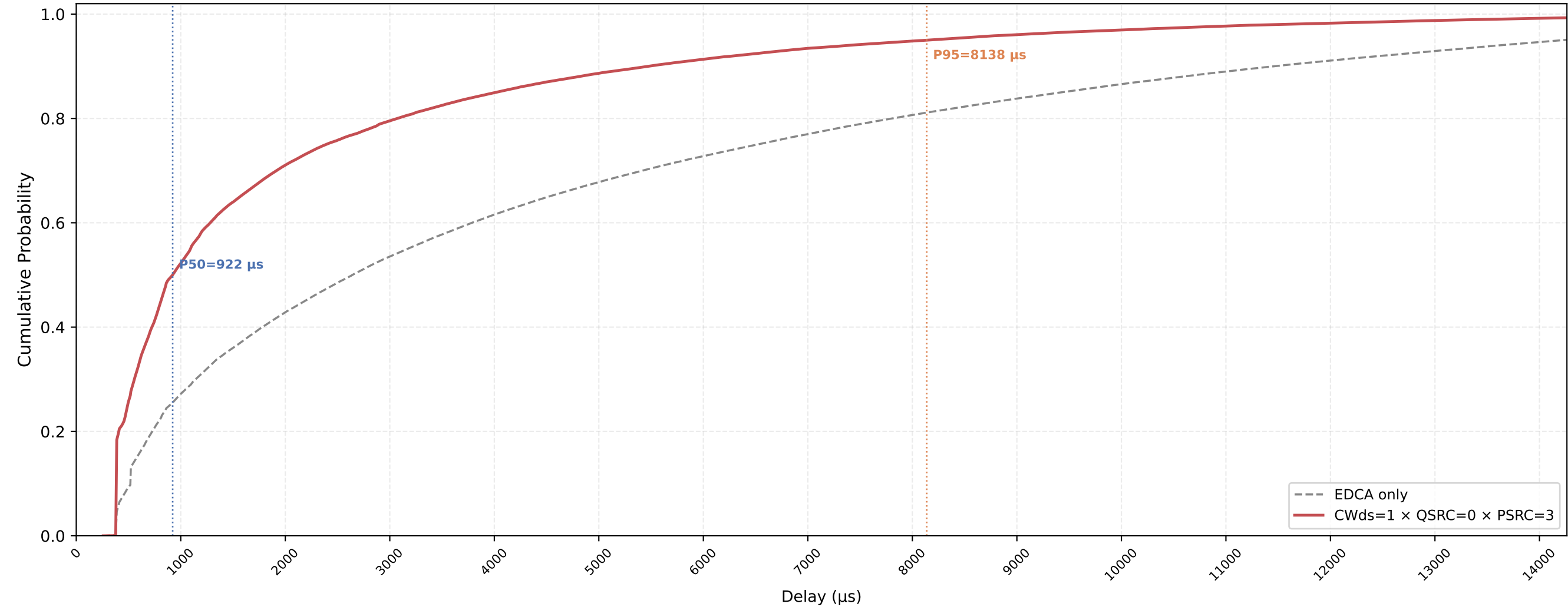
Legacy STA VO Delay CDF — CWds=1 × QSRC=0 × PSRC=3 nSta=30, nPedca=15, 0.5Mbps, avg of 10 runs
