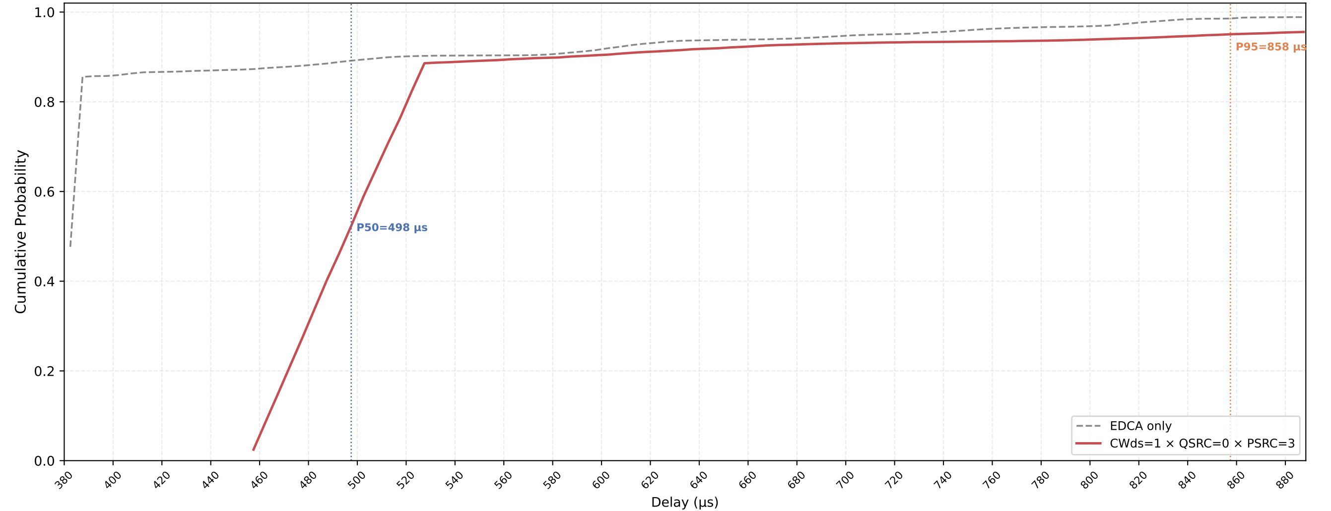
VO (all STAs) Delay CDF — CWds=1 × QSRC=0 × PSRC=3 nSta=30, nPedca=30, 0.1Mbps, avg of 10 runs
