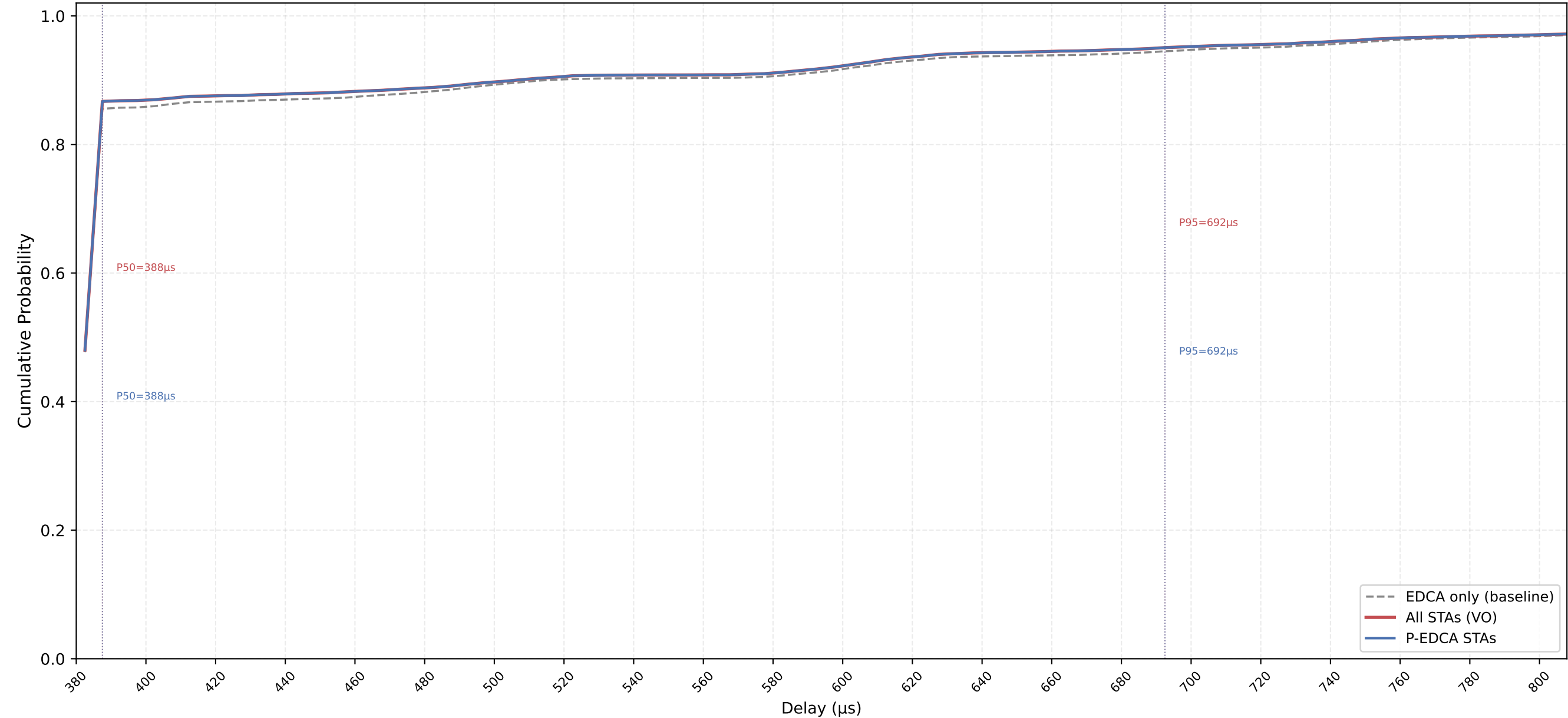
VO Delay CDF — P-EDCA / Legacy / All | CWds=1 × QSRC=1 × PSRC=2 nSta=30, nPedca=30/30, 0.1Mbps, avg of 10 runs
