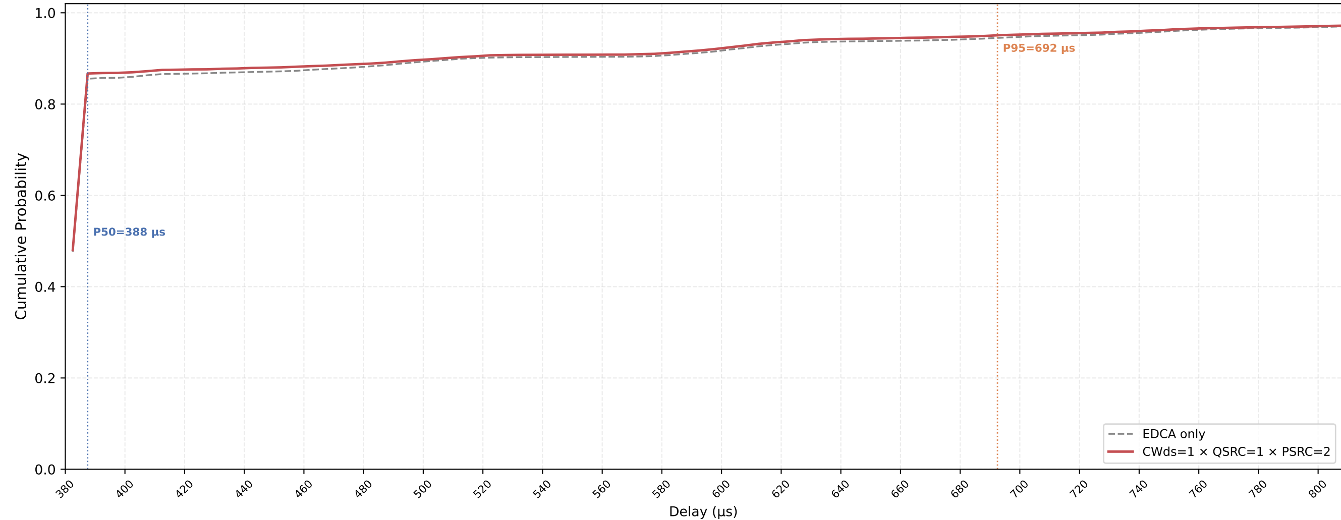
VO (all STAs) Delay CDF — CWds=1 × QSRC=1 × PSRC=2 nSta=30, nPedca=30, 0.1Mbps, avg of 10 runs
