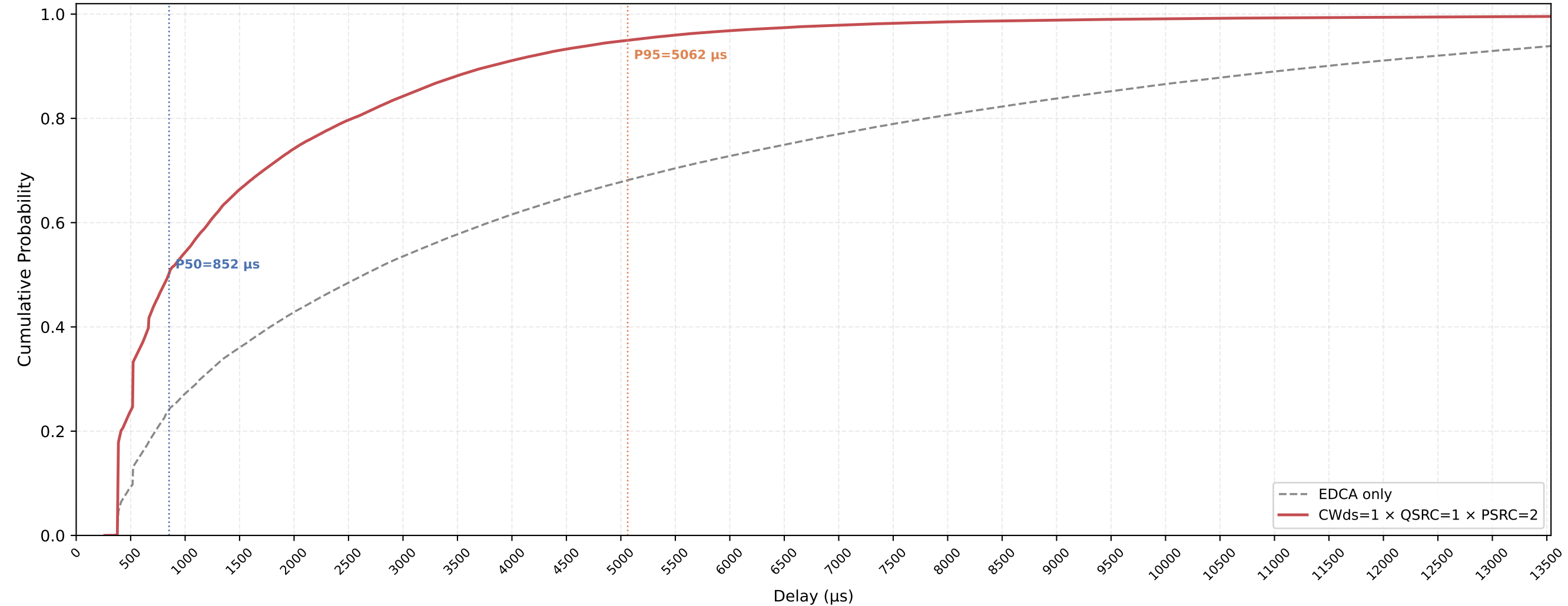
VO (all STAs) Delay CDF — CWds=1 × QSRC=1 × PSRC=2 nSta=30, nPedca=30, 0.5Mbps, avg of 10 runs
