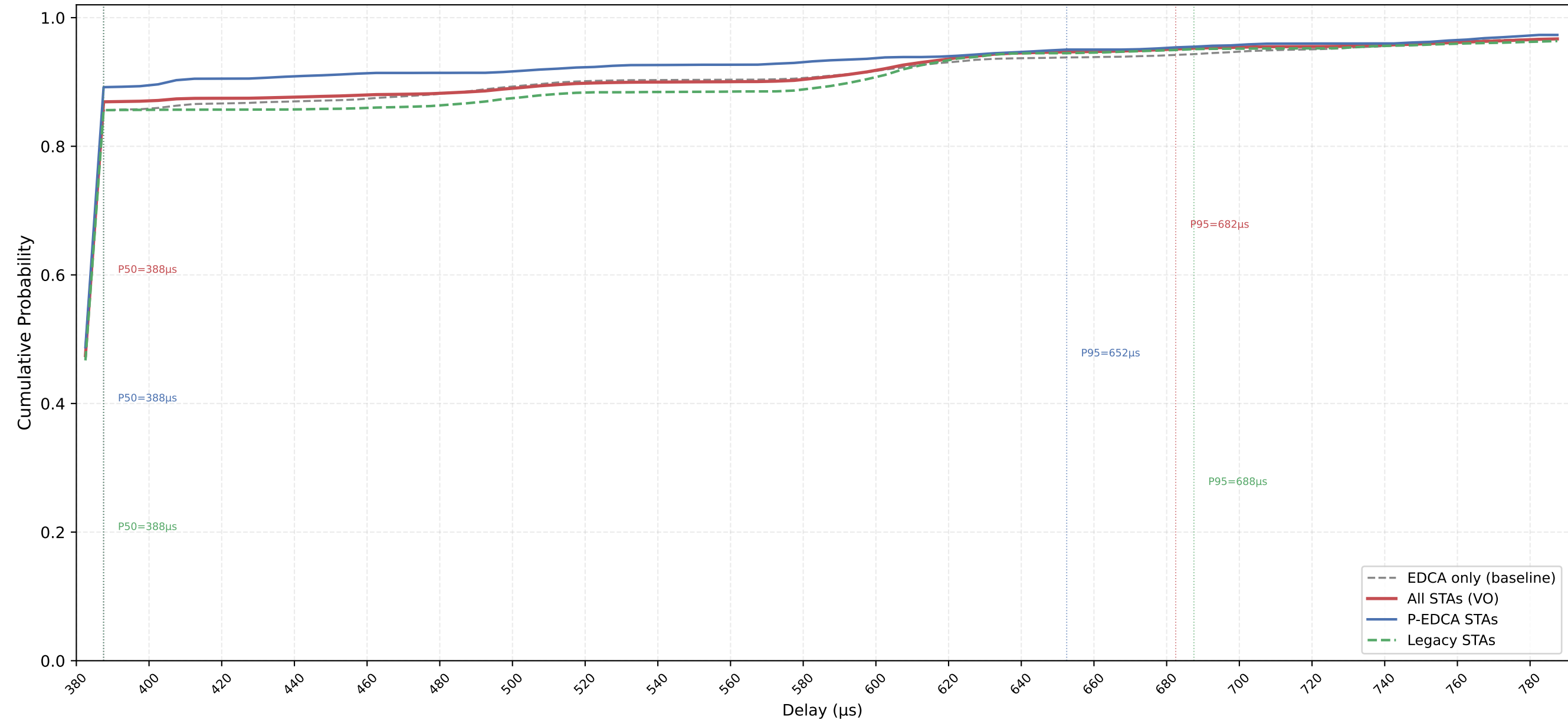
VO Delay CDF — P-EDCA / Legacy / All | CWds=1 × QSRC=1 × PSRC=3 nSta=30, nPedca=15/30, 0.1Mbps, avg of 10 runs
