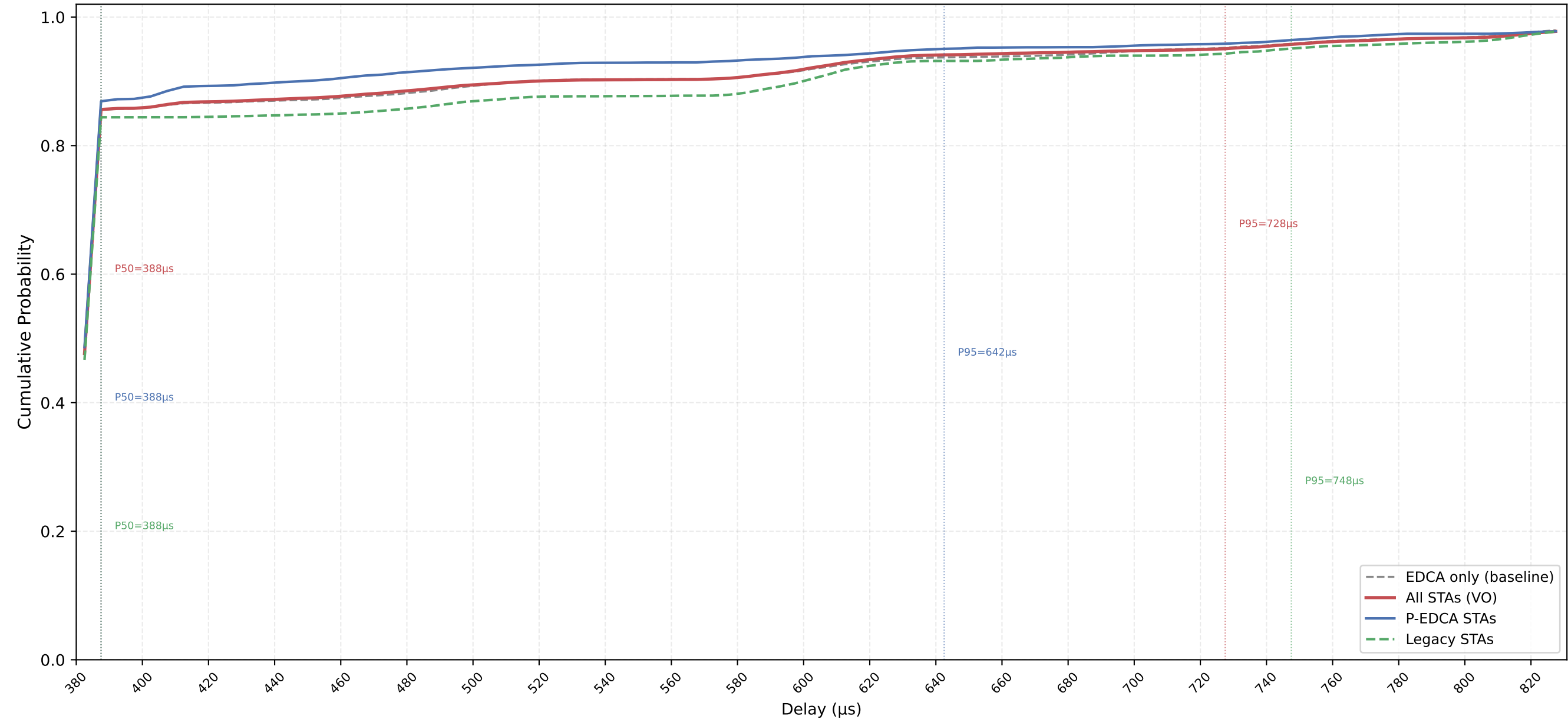
VO Delay CDF — P-EDCA / Legacy / All | CWds=1 × QSRC=2 × PSRC=1 nSta=30, nPedca=15/30, 0.1Mbps, avg of 10 runs
