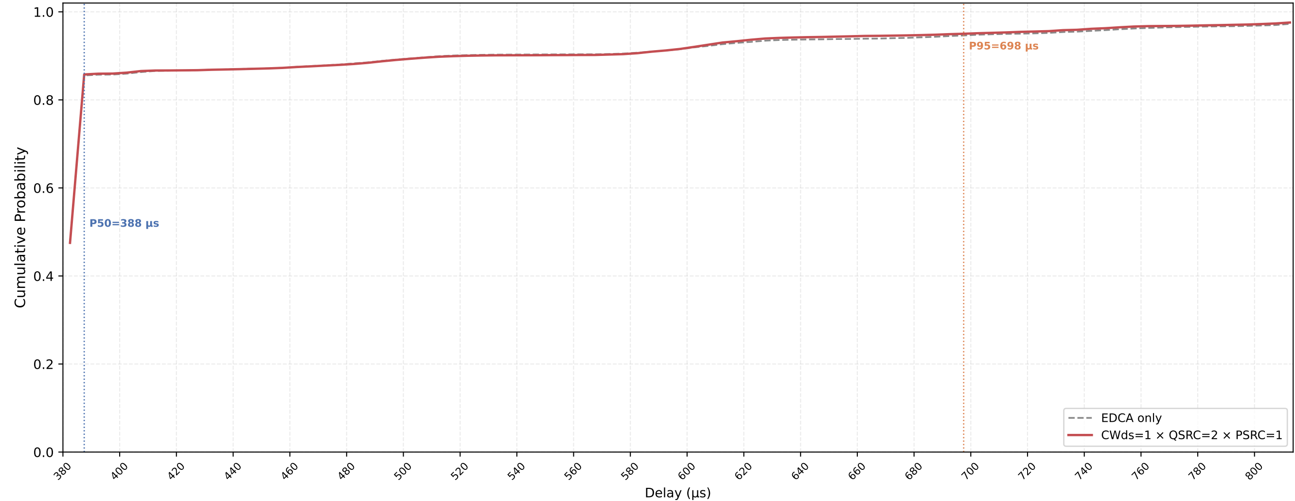
Legacy STA VO Delay CDF — CWds=1 × QSRC=2 × PSRC=1 nSta=30, nPedca=5, 0.1Mbps, avg of 10 runs
