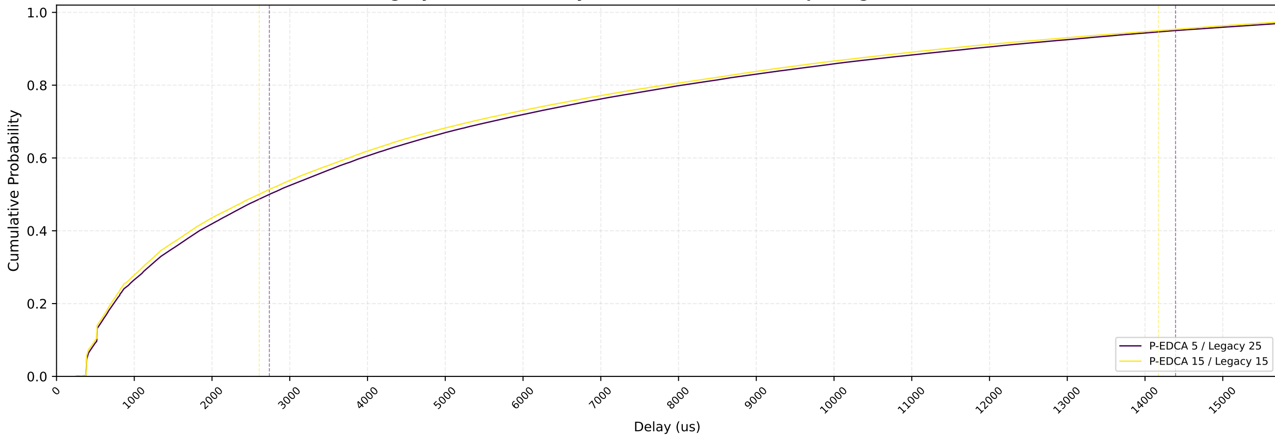
Legacy EDCA STAs Delay CDF — nSta=30, 0.5Mbps, avg of 10 runs
