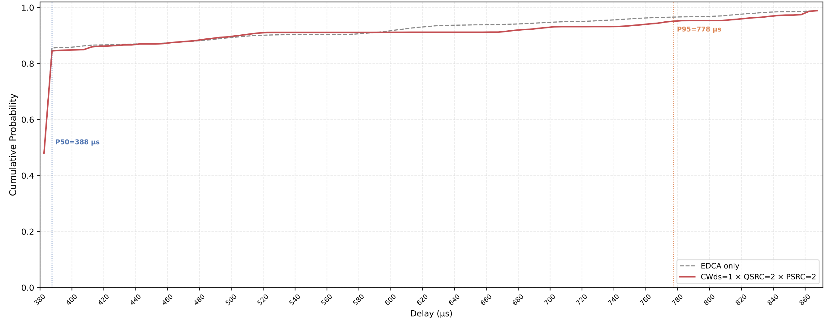
P-EDCA STA VO Delay CDF — CWds=1 × QSRC=2 × PSRC=2 nSta=30, nPedca=5, 0.1Mbps, avg of 10 runs
