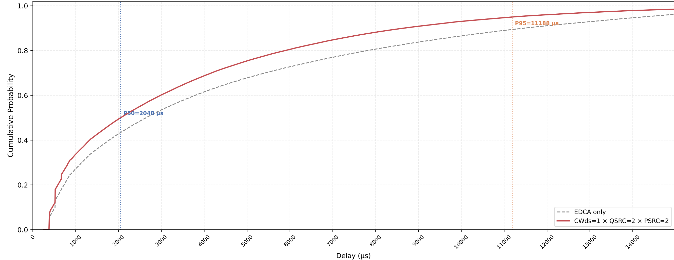
P-EDCA STA VO Delay CDF — CWds=1 × QSRC=2 × PSRC=2 nSta=30, nPedca=30, 0.5Mbps, avg of 10 runs
