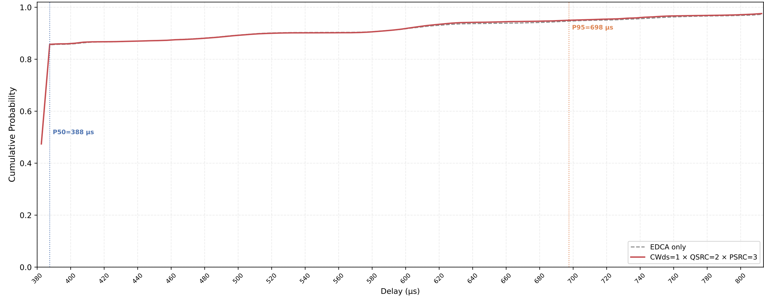
Legacy STA VO Delay CDF — CWds=1 × QSRC=2 × PSRC=3 nSta=30, nPedca=5, 0.1Mbps, avg of 10 runs
