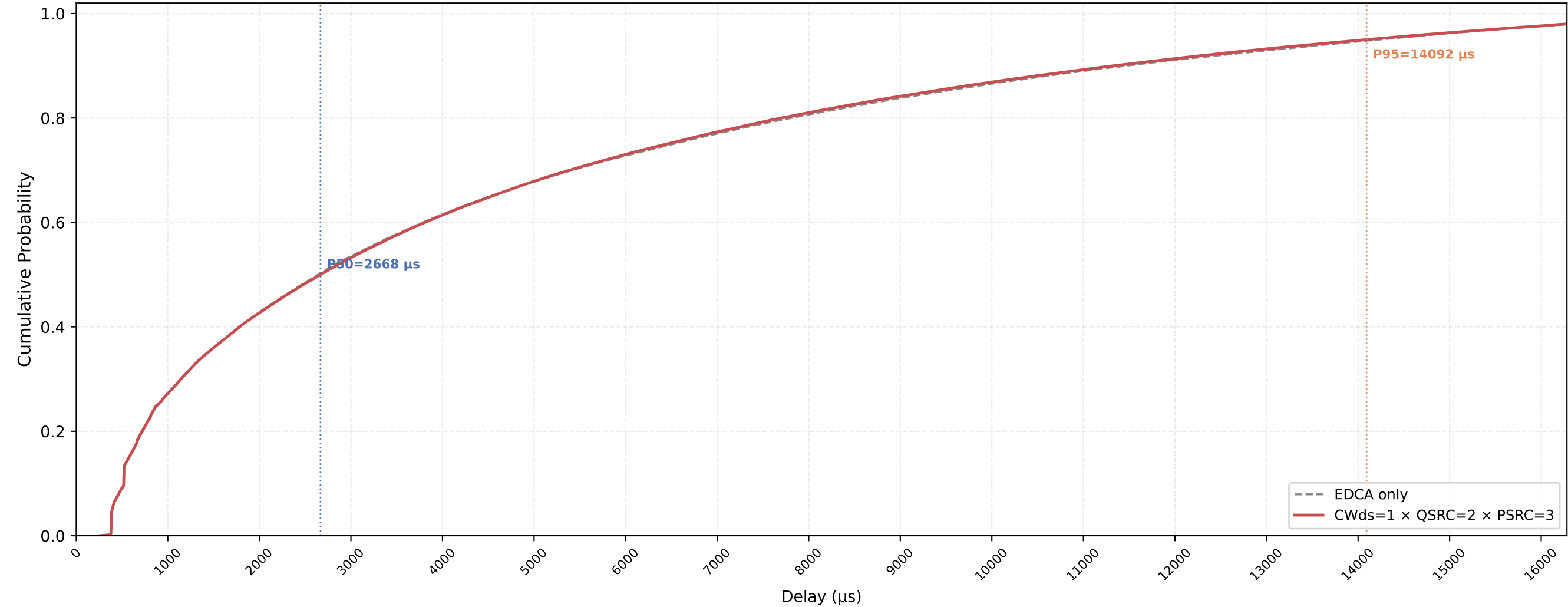
VO (all STAs) Delay CDF — CWds=1 × QSRC=2 × PSRC=3 nSta=30, nPedca=5, 0.5Mbps, avg of 10 runs
