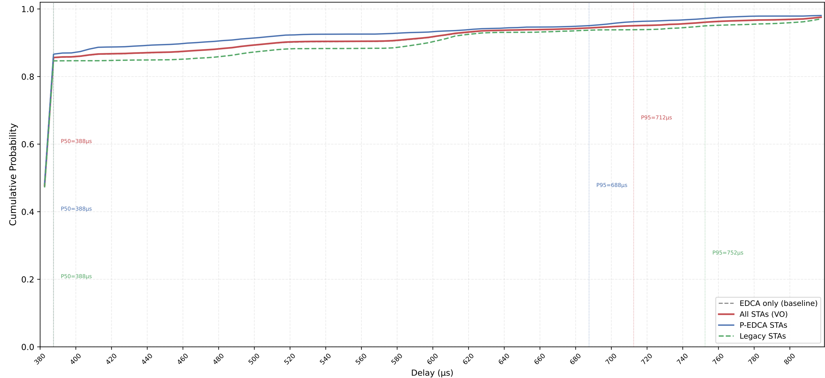
VO Delay CDF — P-EDCA / Legacy / All | CWds=1 × QSRC=3 × PSRC=1 nSta=30, nPedca=15/30, 0.1Mbps, avg of 10 runs
