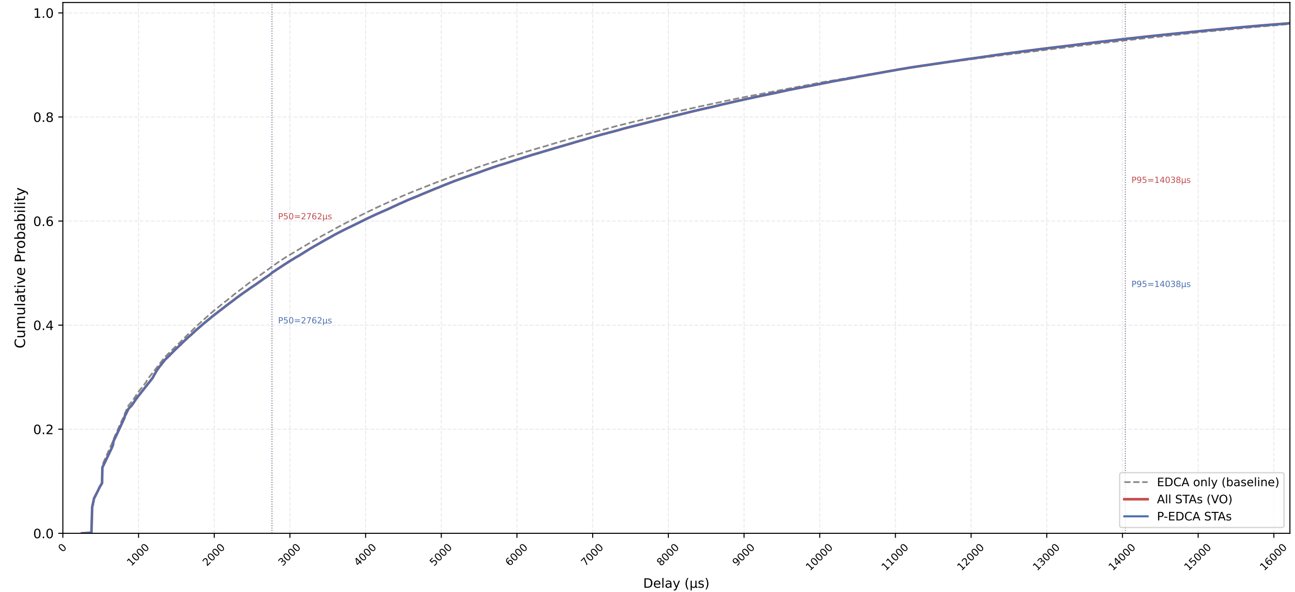
VO Delay CDF — P-EDCA / Legacy / All | CWds=1 × QSRC=3 × PSRC=1 nSta=30, nPedca=30/30, 0.5Mbps, avg of 10 runs
