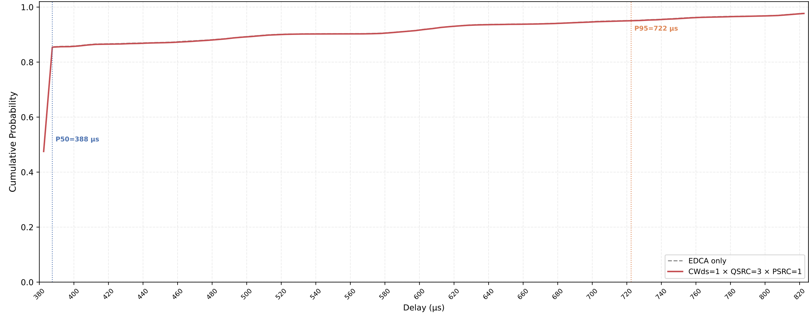
VO (all STAs) Delay CDF — CWds=1 × QSRC=3 × PSRC=1 nSta=30, nPedca=5, 0.1Mbps, avg of 10 runs
