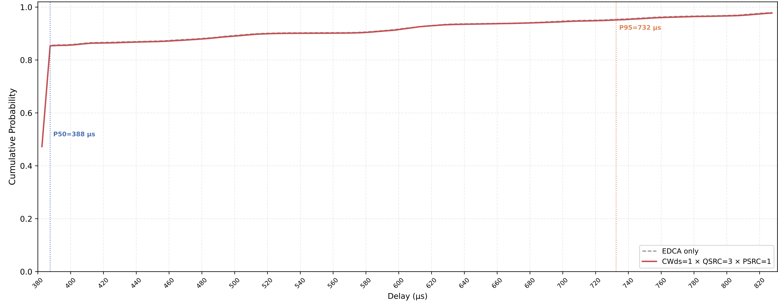
VO (all STAs) Delay CDF — CWds=1 × QSRC=3 × PSRC=1 nSta=30, nPedca=30, 0.1Mbps, avg of 10 runs
