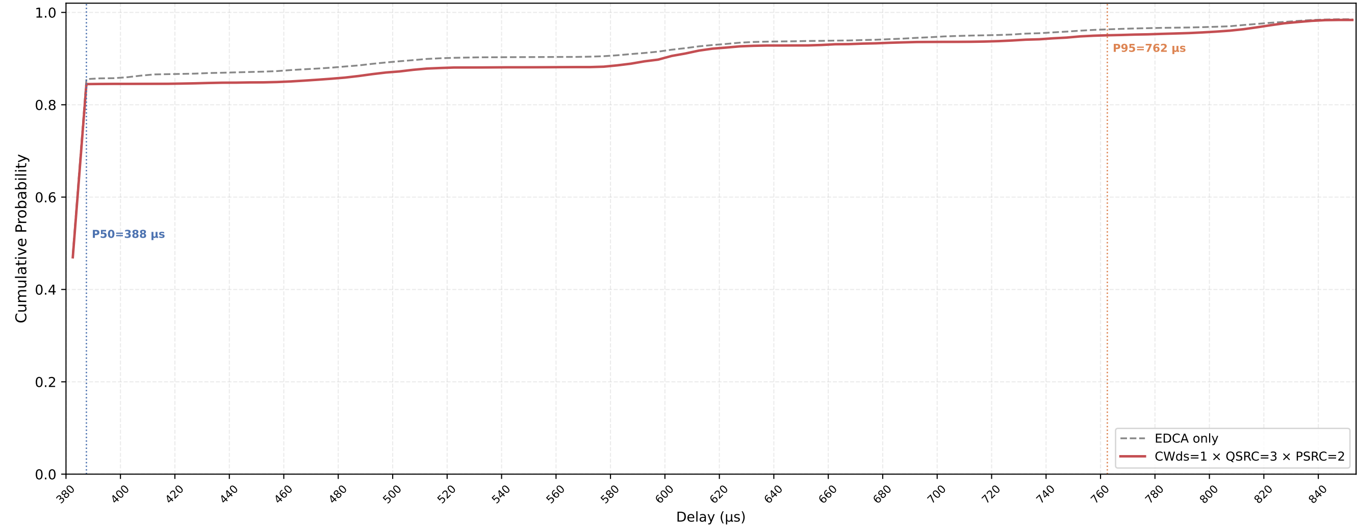
Legacy STA VO Delay CDF — CWds=1 × QSRC=3 × PSRC=2 nSta=30, nPedca=15, 0.1Mbps, avg of 10 runs
