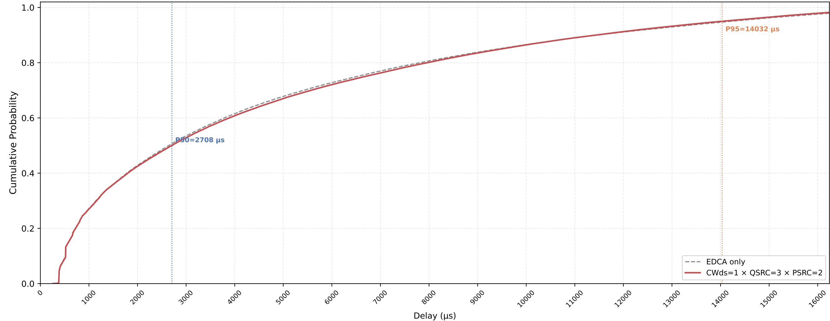
VO (all STAs) Delay CDF — CWds=1 × QSRC=3 × PSRC=2 nSta=30, nPedca=15, 0.5Mbps, avg of 10 runs
