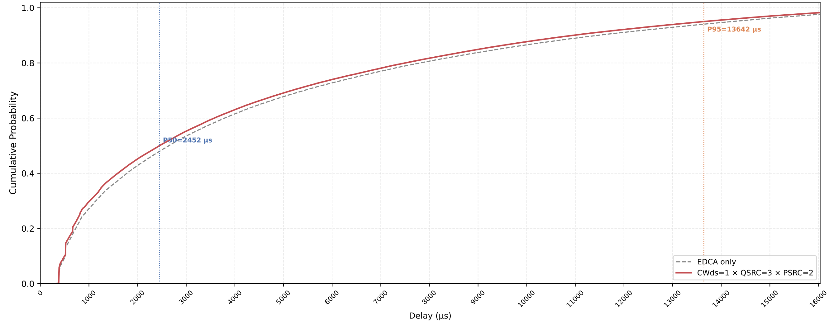
VO (all STAs) Delay CDF — CWds=1 × QSRC=3 × PSRC=2 nSta=30, nPedca=30, 0.5Mbps, avg of 10 runs
