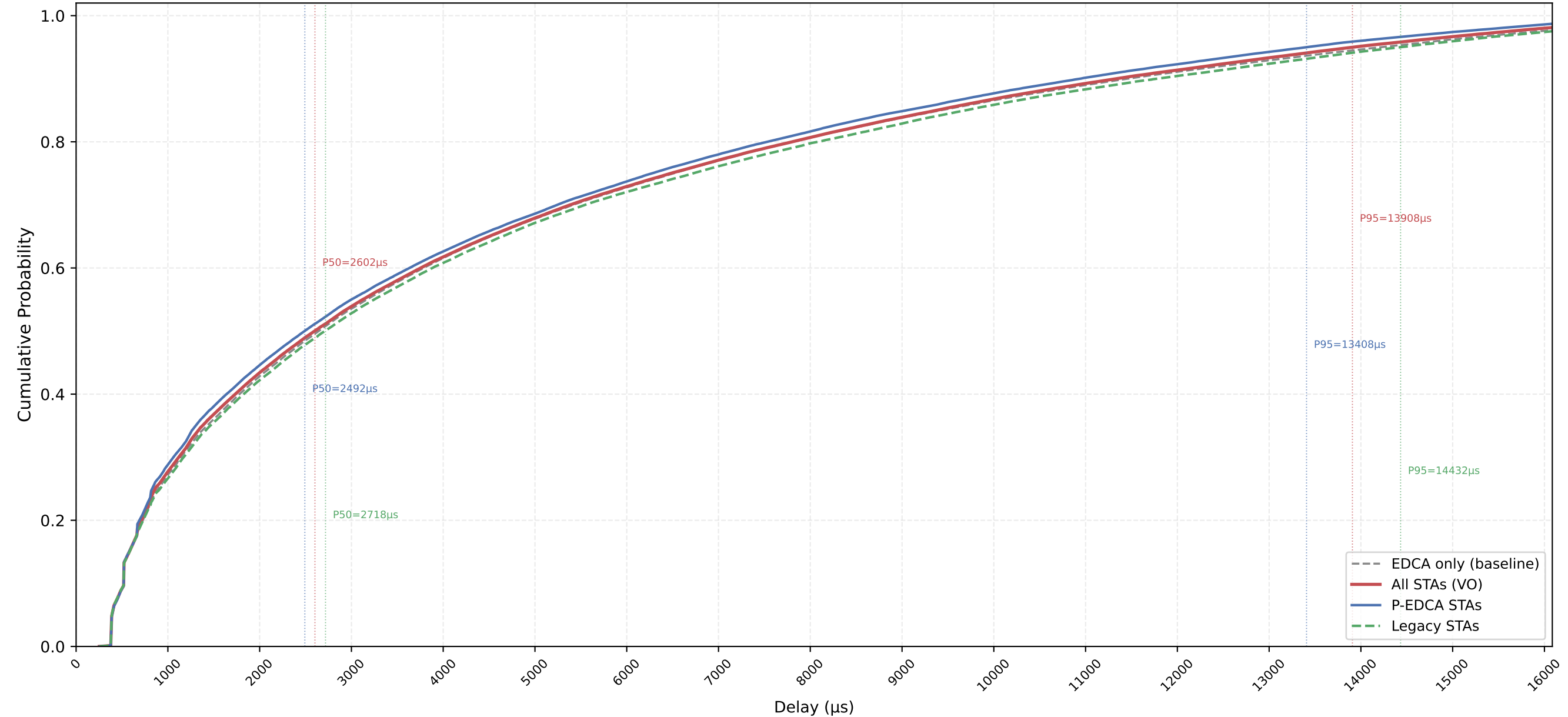
VO Delay CDF — P-EDCA / Legacy / All | CWds=1 × QSRC=3 × PSRC=3 nSta=30, nPedca=15/30, 0.5Mbps, avg of 10 runs
