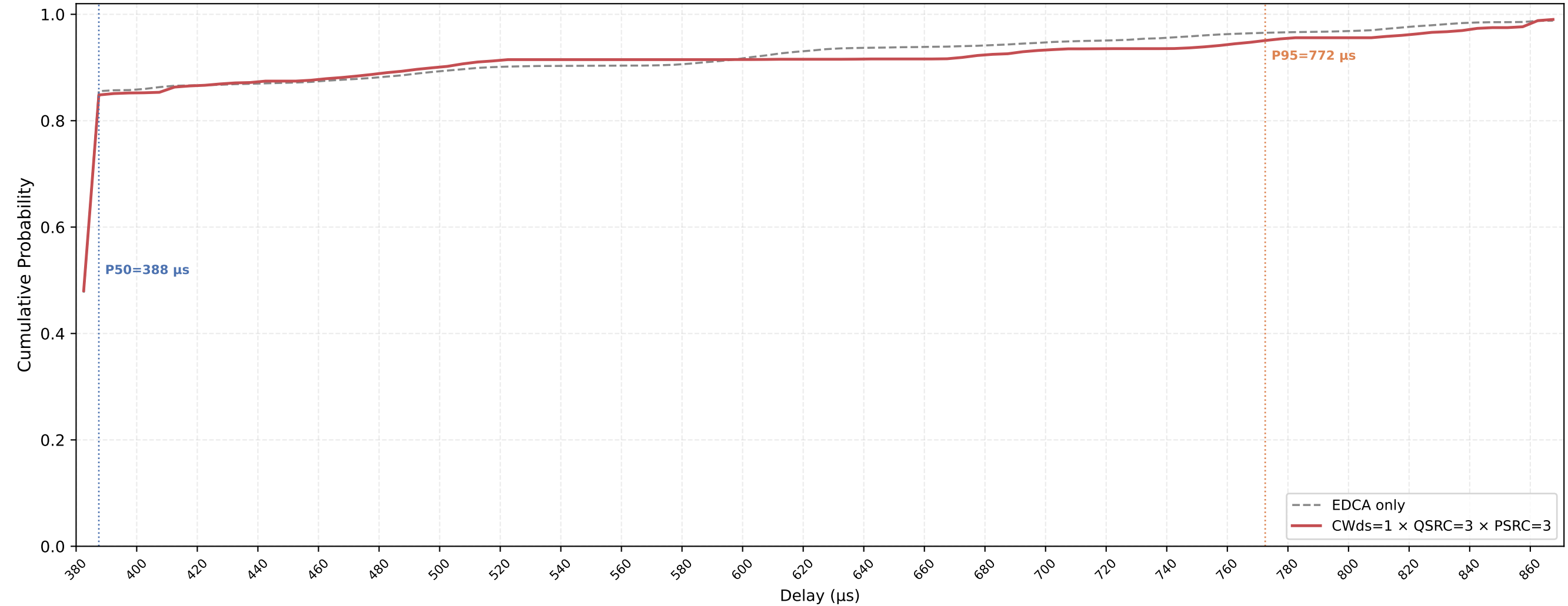
P-EDCA STA VO Delay CDF — CWds=1 × QSRC=3 × PSRC=3 nSta=30, nPedca=5, 0.1Mbps, avg of 10 runs
