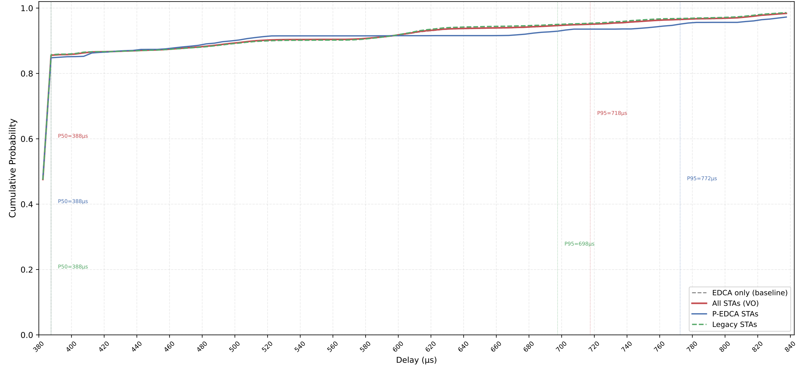
VO Delay CDF — P-EDCA / Legacy / All | CWds=1 × QSRC=4 × PSRC=1 nSta=30, nPedca=5/30, 0.1Mbps, avg of 10 runs
