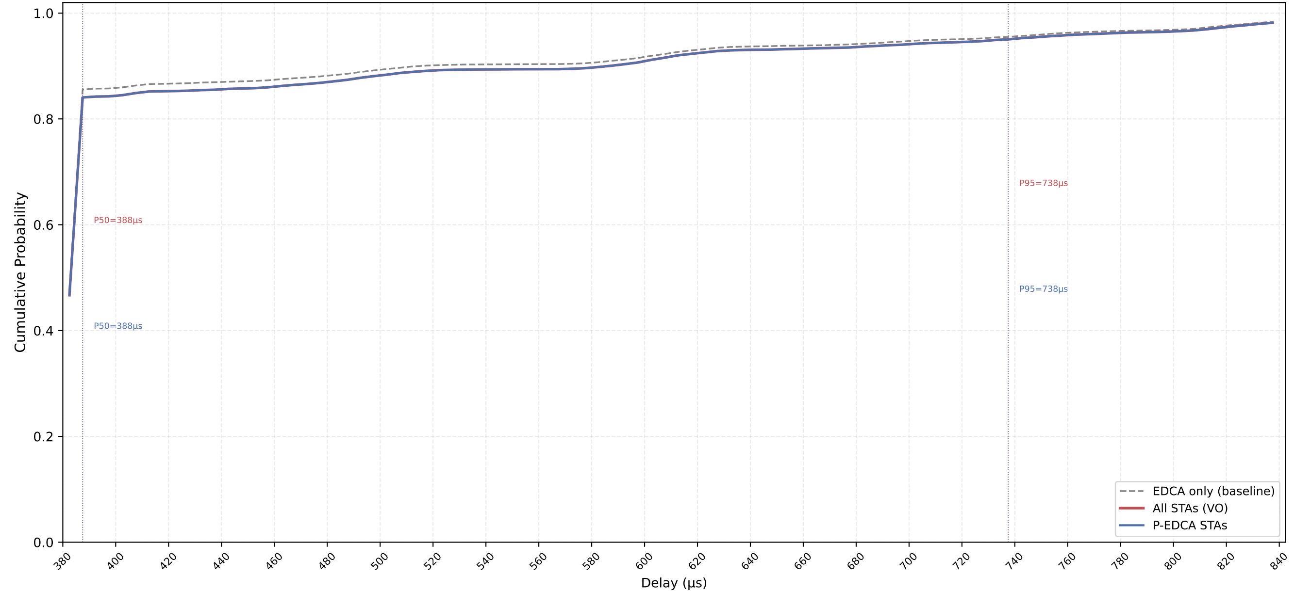
VO Delay CDF — P-EDCA / Legacy / All | CWds=1 × QSRC=4 × PSRC=1 nSta=30, nPedca=30/30, 0.1Mbps, avg of 10 runs
