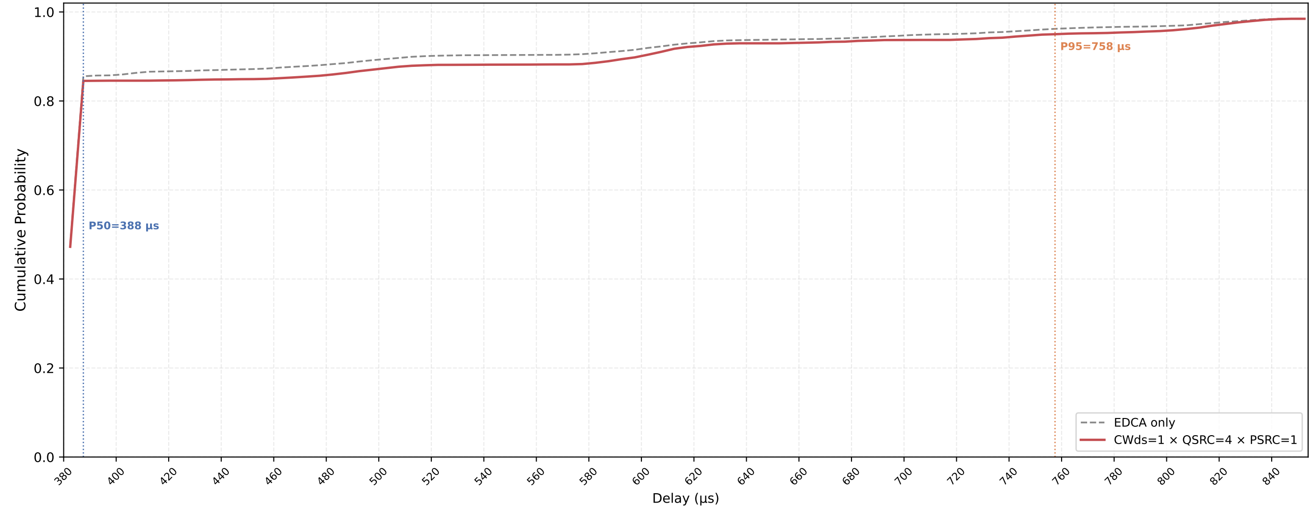
Legacy STA VO Delay CDF — CWds=1 × QSRC=4 × PSRC=1 nSta=30, nPedca=15, 0.1Mbps, avg of 10 runs
