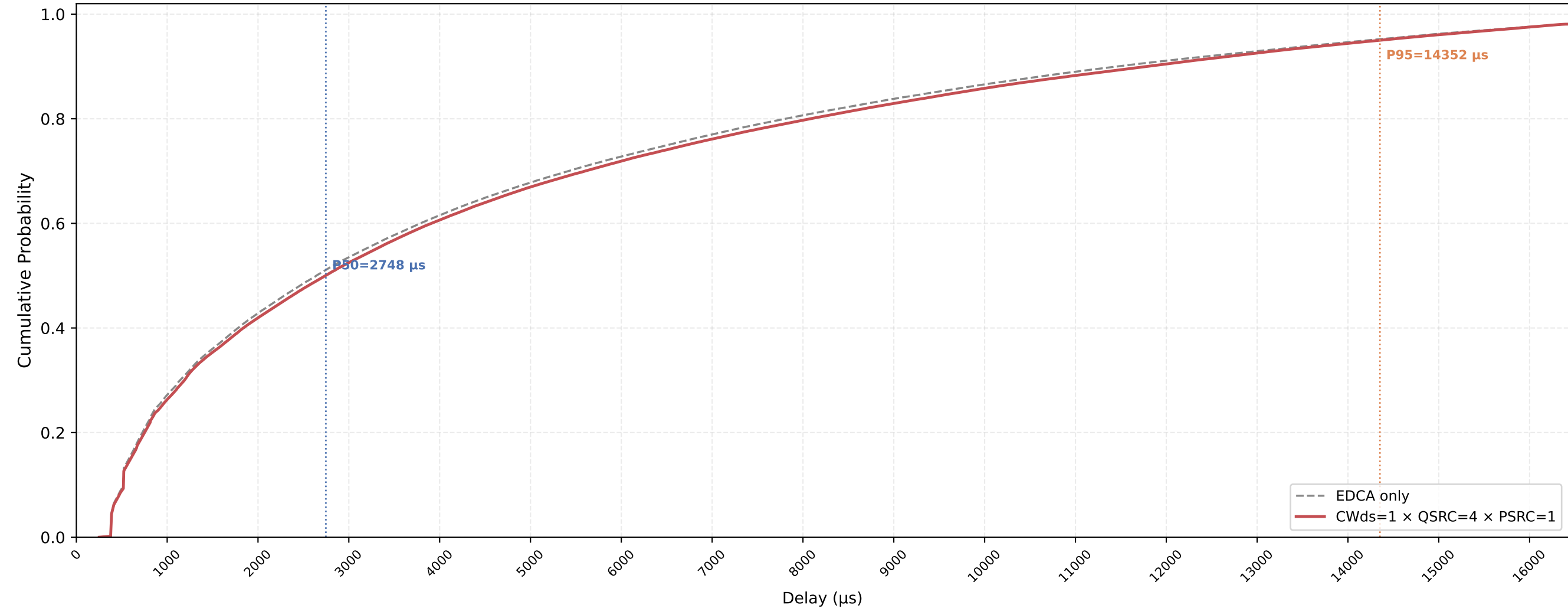
VO (all STAs) Delay CDF — CWds=1 × QSRC=4 × PSRC=1 nSta=30, nPedca=15, 0.5Mbps, avg of 10 runs
