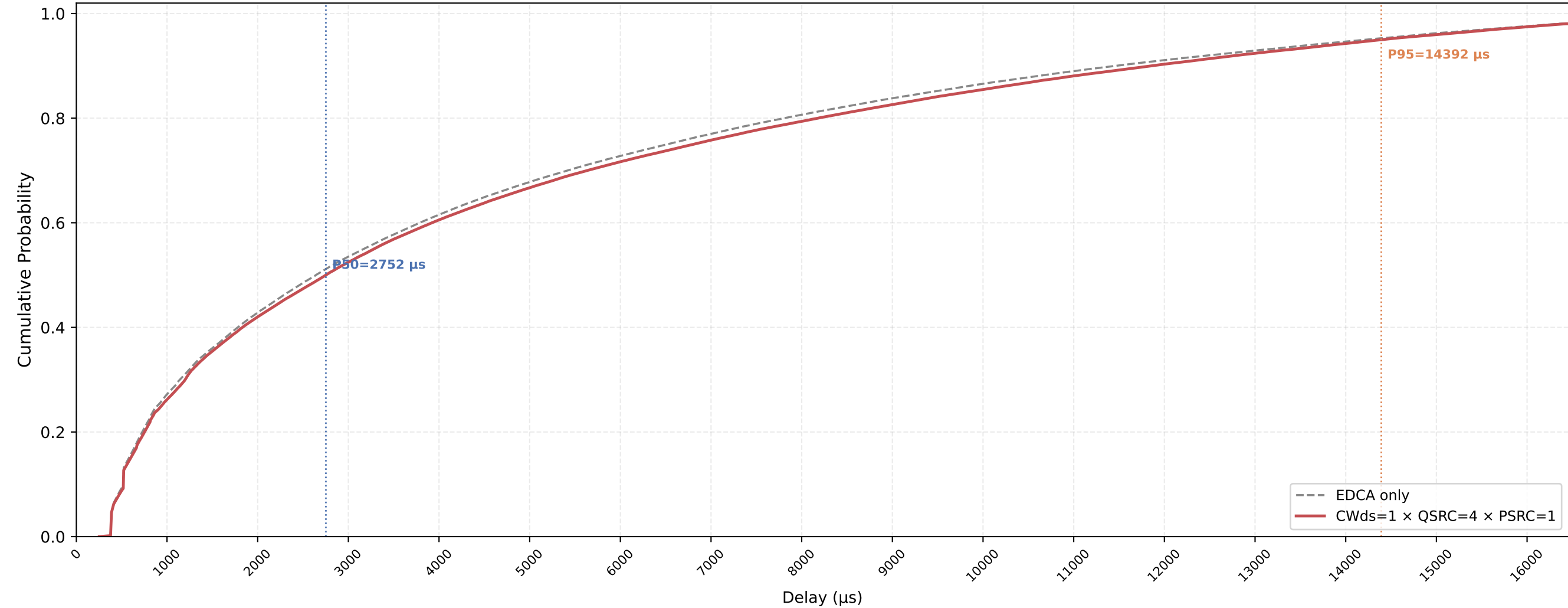
VO (all STAs) Delay CDF — CWds=1 × QSRC=4 × PSRC=1 nSta=30, nPedca=30, 0.5Mbps, avg of 10 runs
