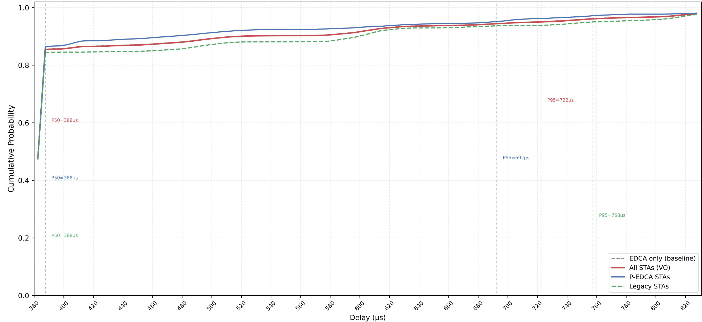
VO Delay CDF — P-EDCA / Legacy / All | CWds=1 × QSRC=4 × PSRC=2 nSta=30, nPedca=15/30, 0.1Mbps, avg of 10 runs
