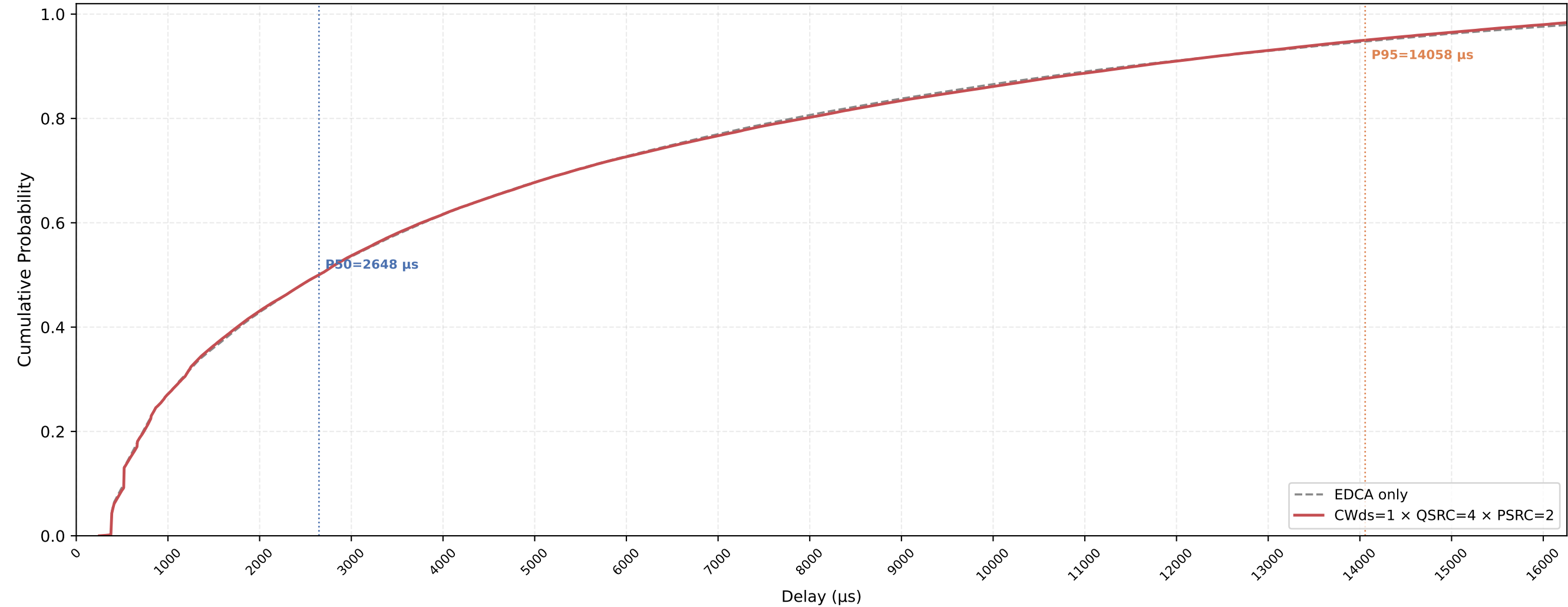
P-EDCA STA VO Delay CDF — CWds=1 × QSRC=4 × PSRC=2 nSta=30, nPedca=15, 0.5Mbps, avg of 10 runs
