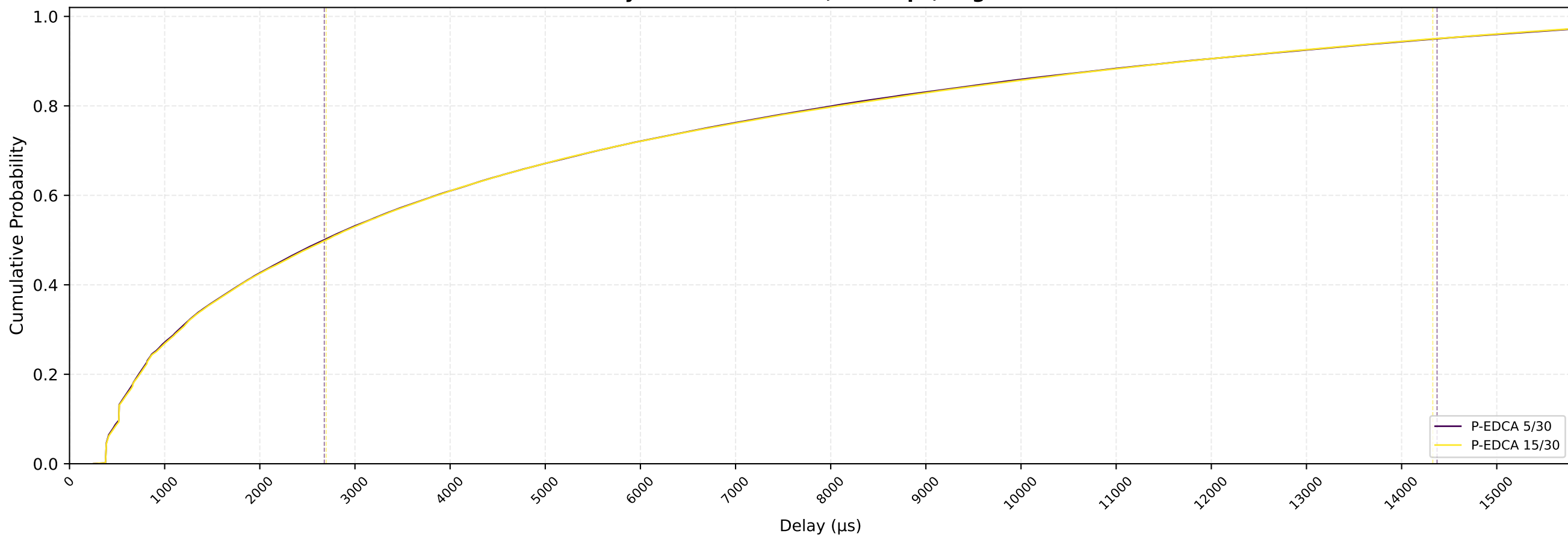
VO Delay CDF — nSta=30, 0.5Mbps, avg of 10 runs
