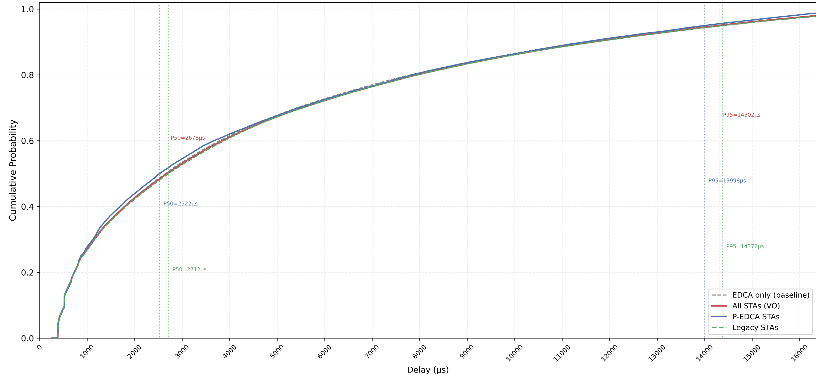
VO Delay CDF — P-EDCA / Legacy / All | CWds=1 × QSRC=4 × PSRC=3 nSta=30, nPedca=5/30, 0.5Mbps, avg of 10 runs
