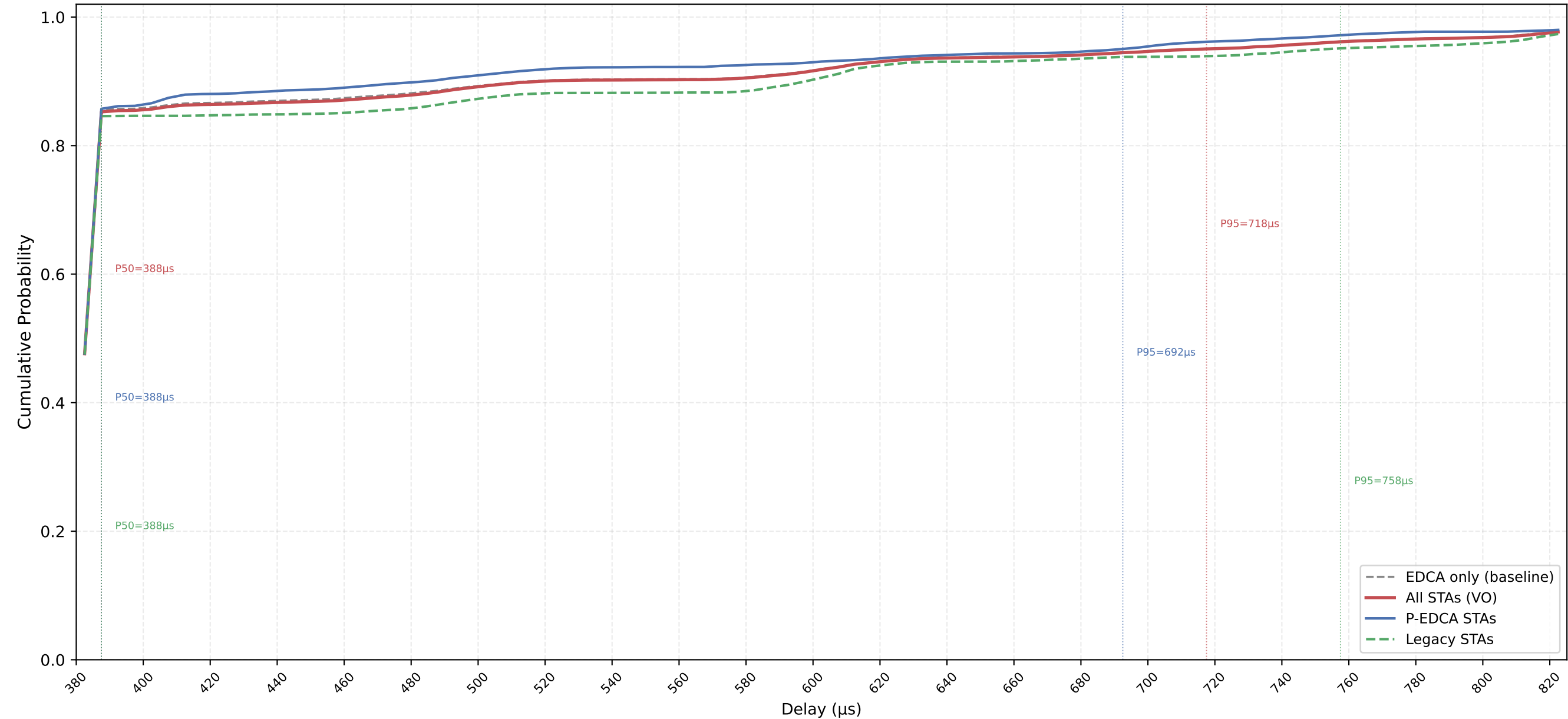
VO Delay CDF — P-EDCA / Legacy / All | CWds=1 × QSRC=4 × PSRC=3 nSta=30, nPedca=15/30, 0.1Mbps, avg of 10 runs
