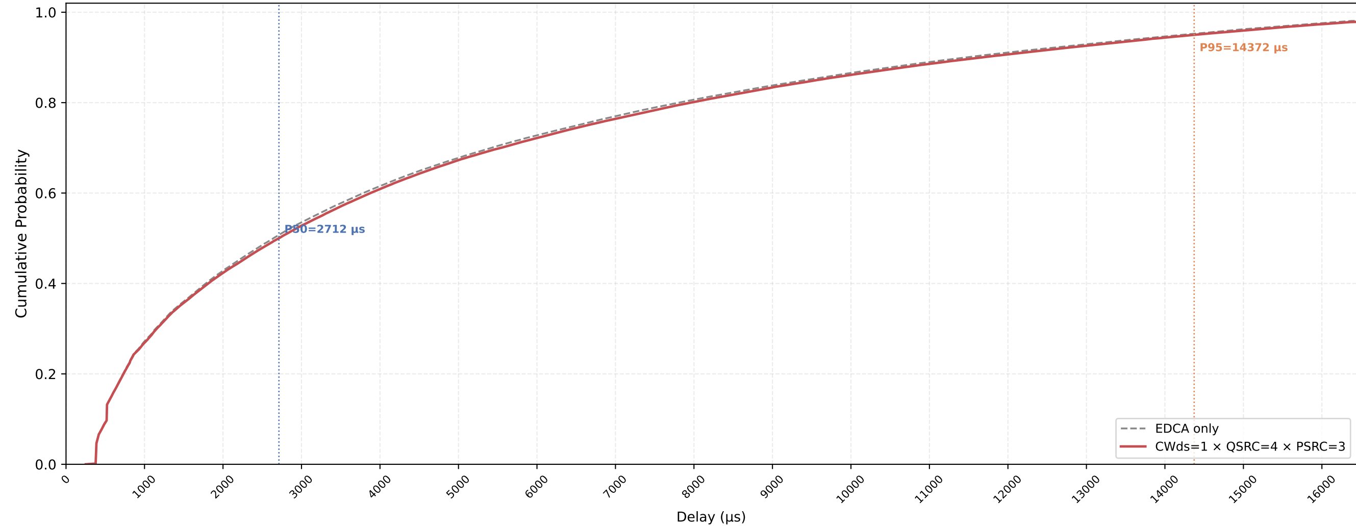
Legacy STA VO Delay CDF — CWds=1 × QSRC=4 × PSRC=3 nSta=30, nPedca=5, 0.5Mbps, avg of 10 runs
