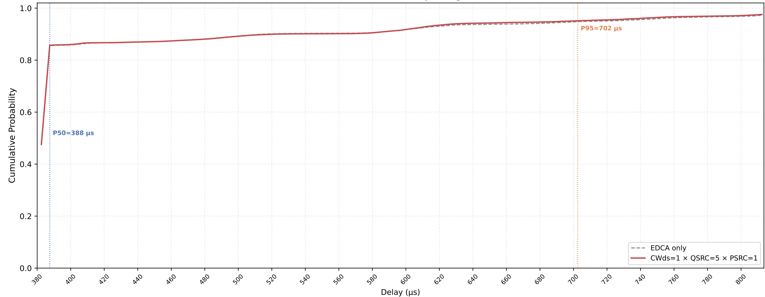
Legacy STA VO Delay CDF — CWds=1 × QSRC=5 × PSRC=1 nSta=30, nPedca=5, 0.1Mbps, avg of 10 runs
