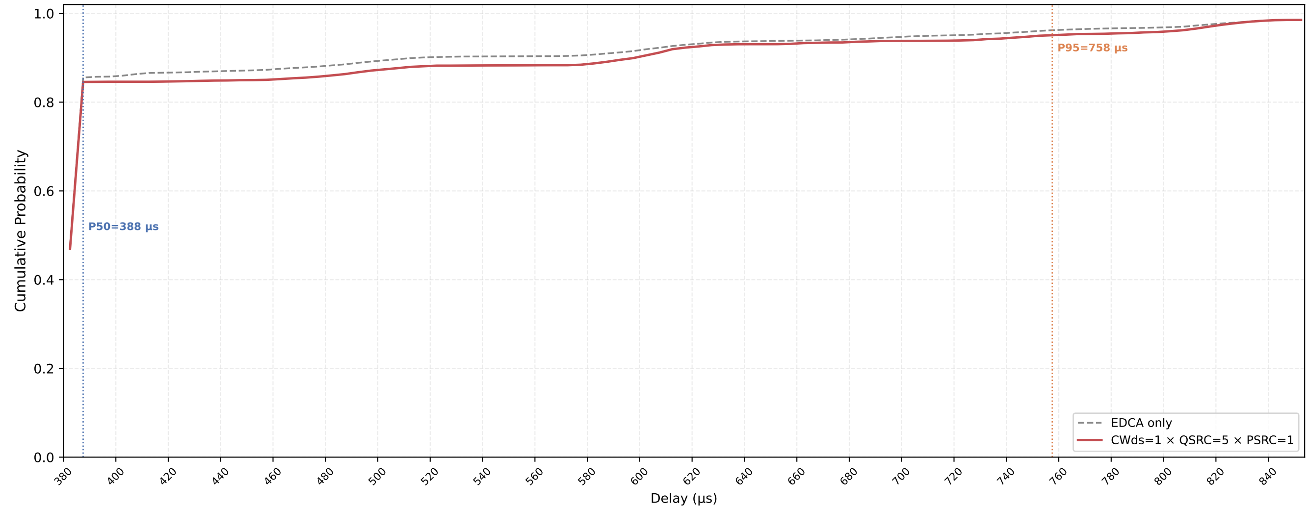
Legacy STA VO Delay CDF — CWds=1 × QSRC=5 × PSRC=1 nSta=30, nPedca=15, 0.1Mbps, avg of 10 runs
