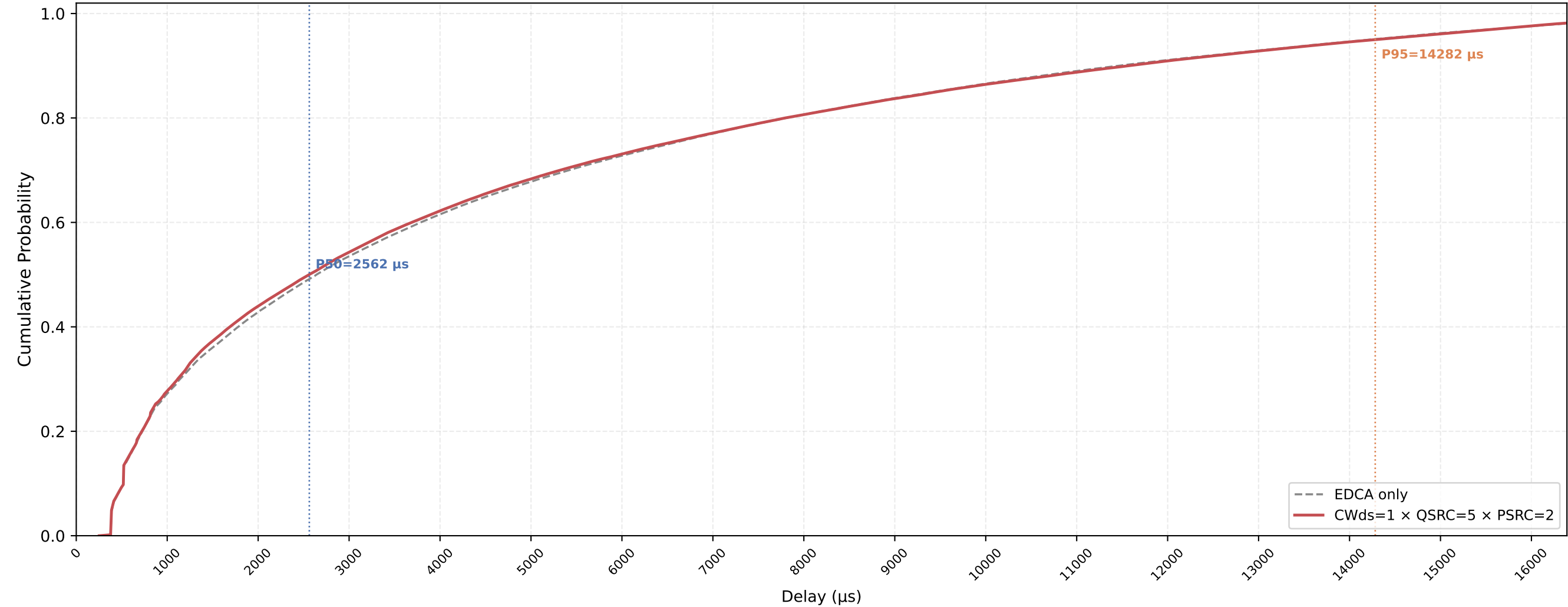
VO (all STAs) Delay CDF — CWds=1 × QSRC=5 × PSRC=2 nSta=30, nPedca=30, 0.5Mbps, avg of 10 runs
