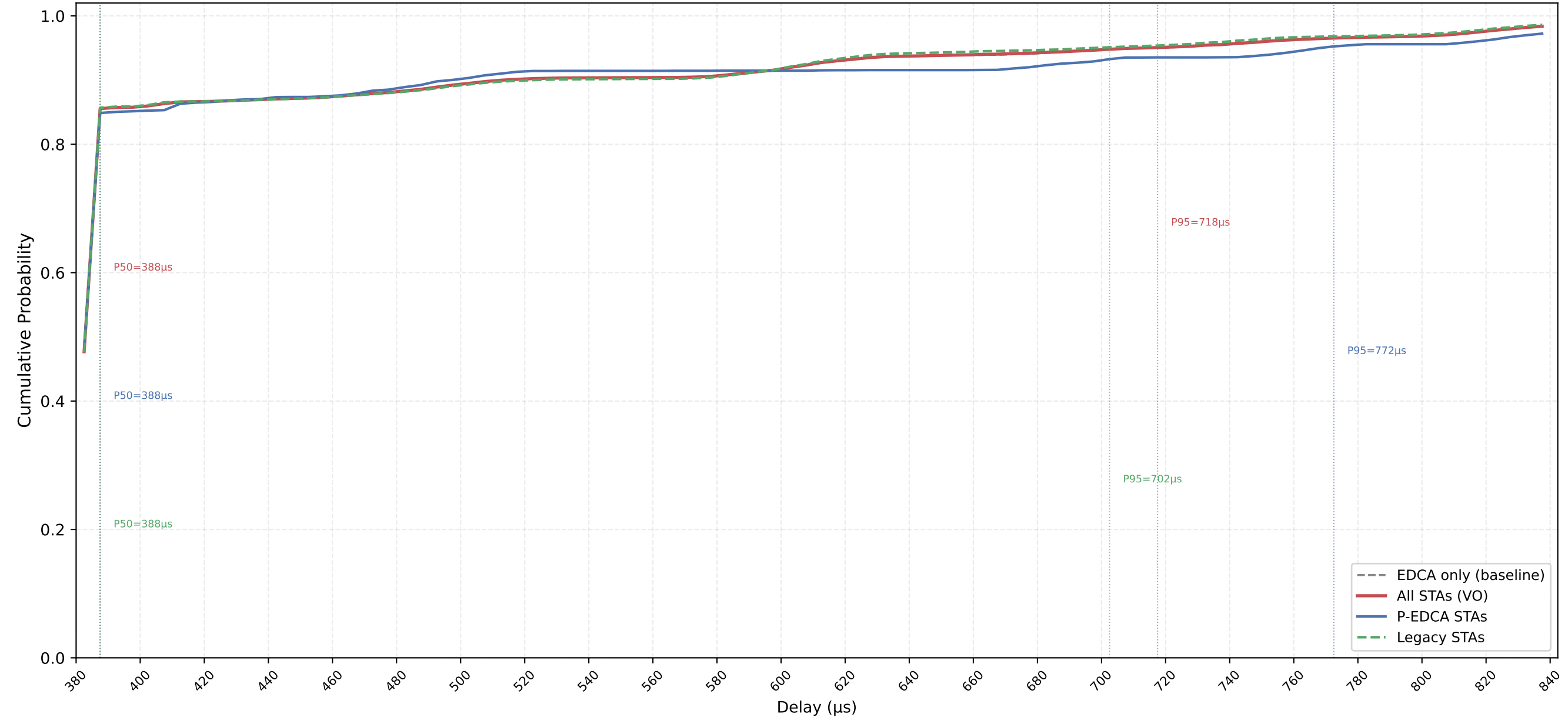
VO Delay CDF — P-EDCA / Legacy / All | CWds=1 × QSRC=5 × PSRC=3 nSta=30, nPedca=5/30, 0.1Mbps, avg of 10 runs
