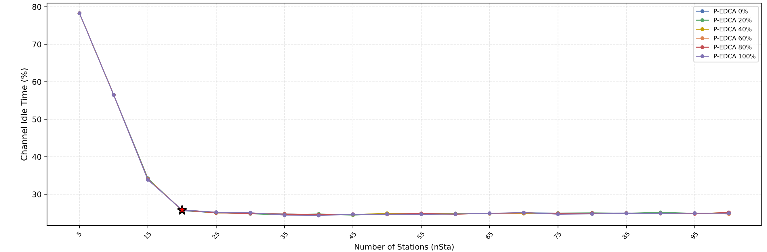
Channel Idle Time vs nSta — (Red Star = Current nSta=20)
