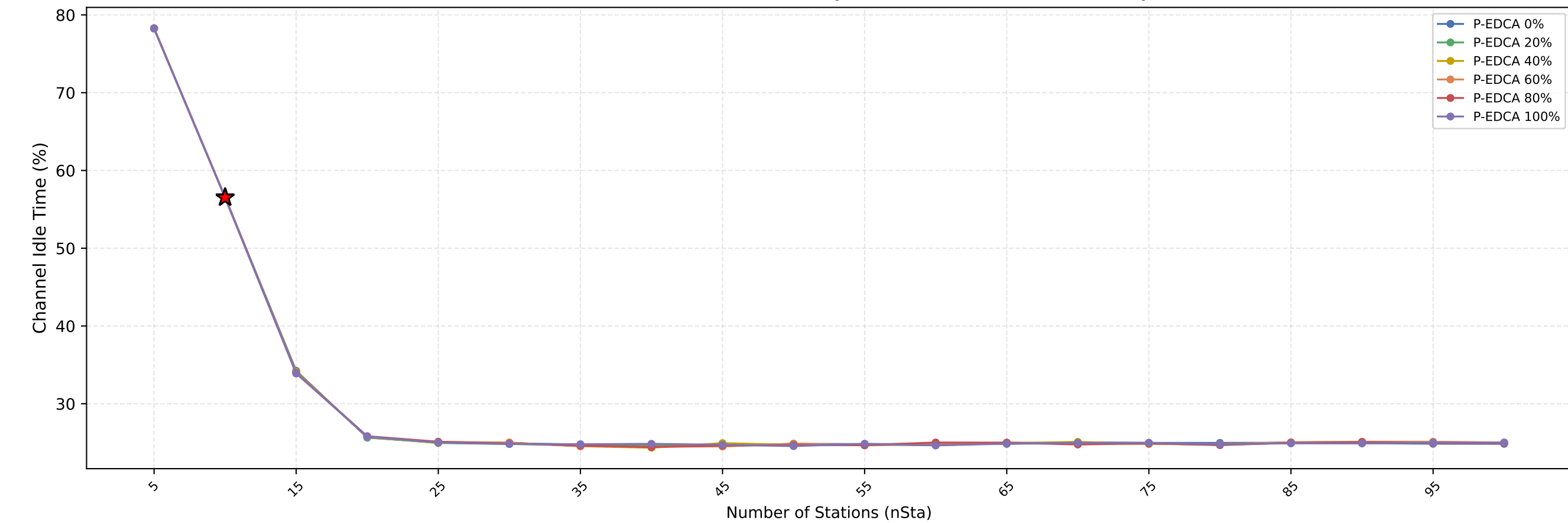
Channel Idle Time vs nSta — (Red Star = Current nSta=10)
