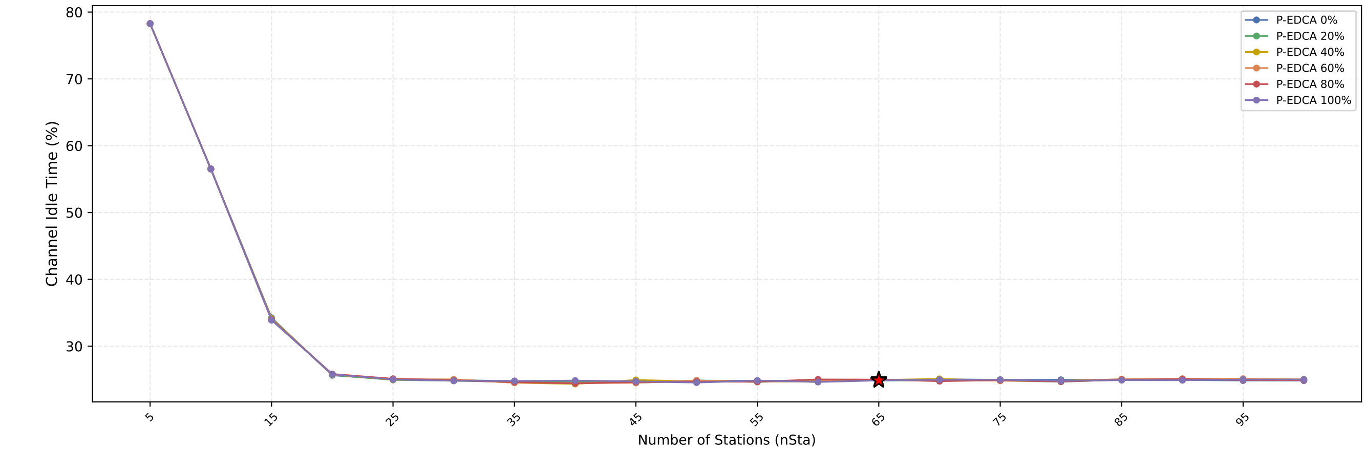
Channel Idle Time vs nSta — (Red Star = Current nSta=65)
