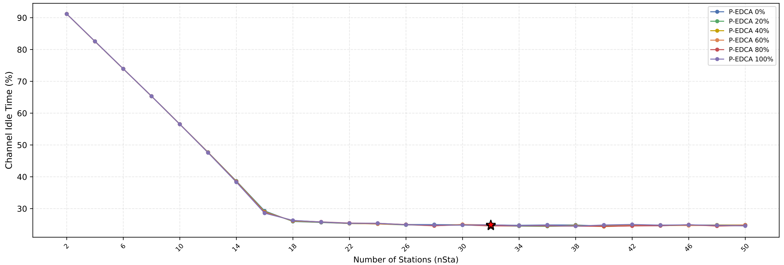
Channel Idle Time vs nSta — (Red Star = Current nSta=32)
