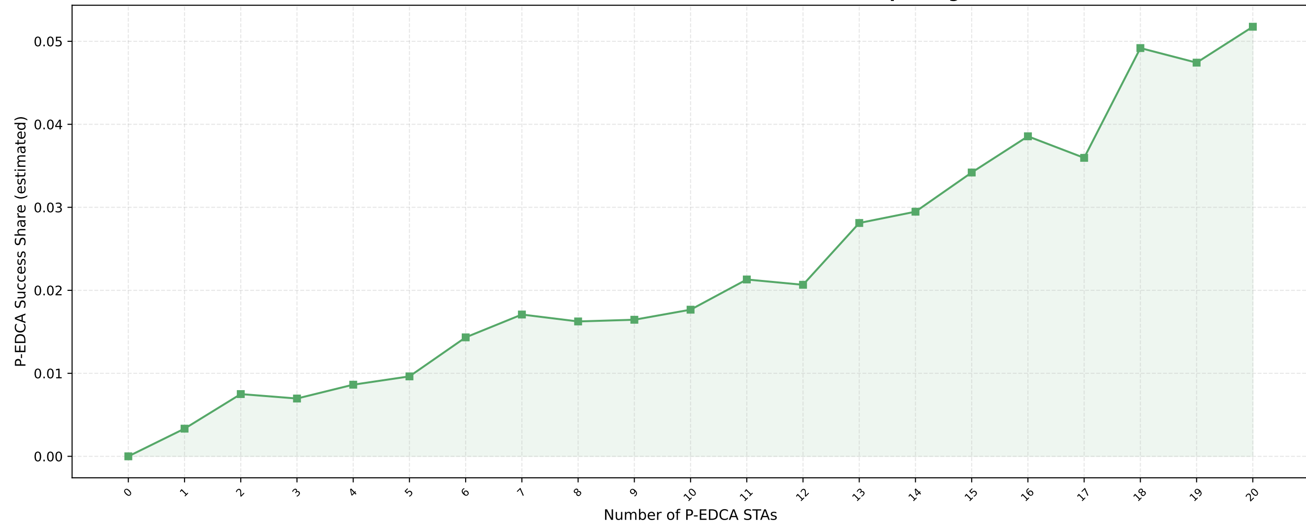
Estimated P-EDCA Success / Total Success — nSta=20, 1Mbps (avg of 10 runs)
