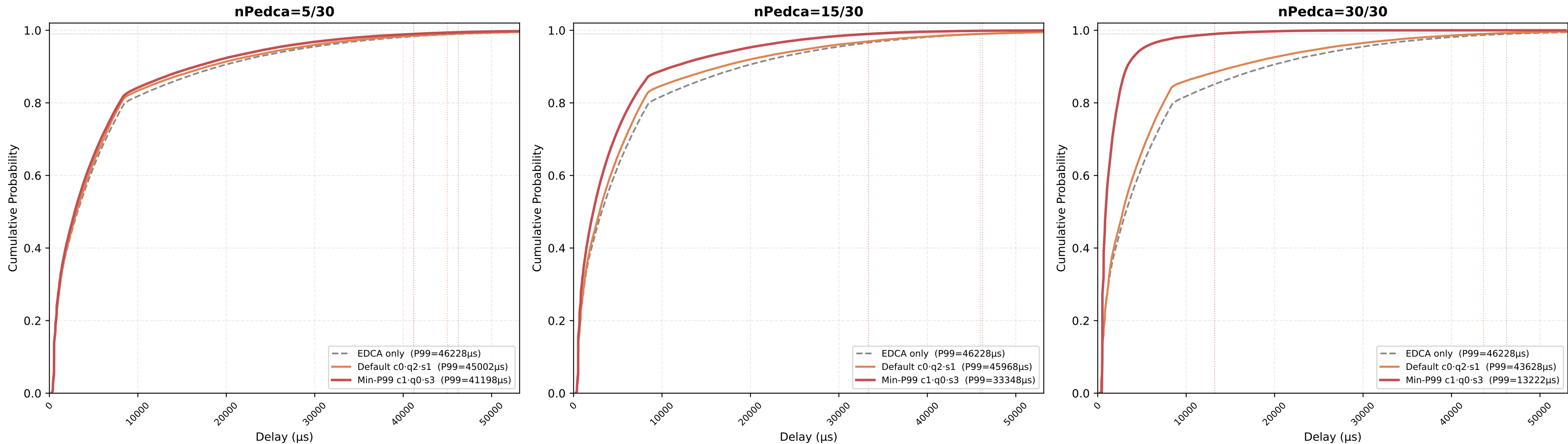
All STAs — Min-P99 vs Default (c0·q2·s1) vs EDCA-only | nSta=30, 1Mbps, 10 runs avg
