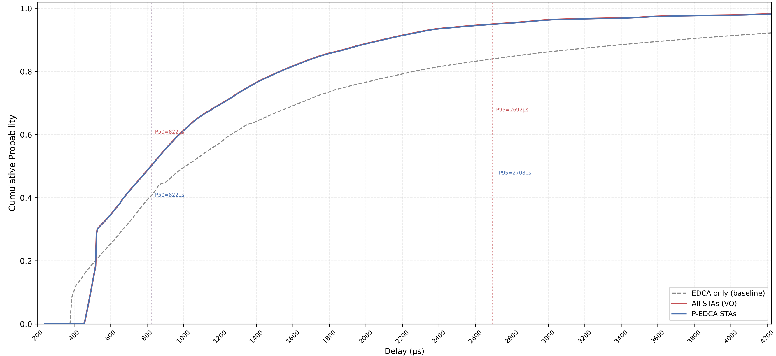
VO Delay CDF — P-EDCA / Legacy / All | CWds=0 × QSRC=0 × PSRC=1 nSta=30, nPedca=30/30, 0.5Mbps, avg of 10 runs
