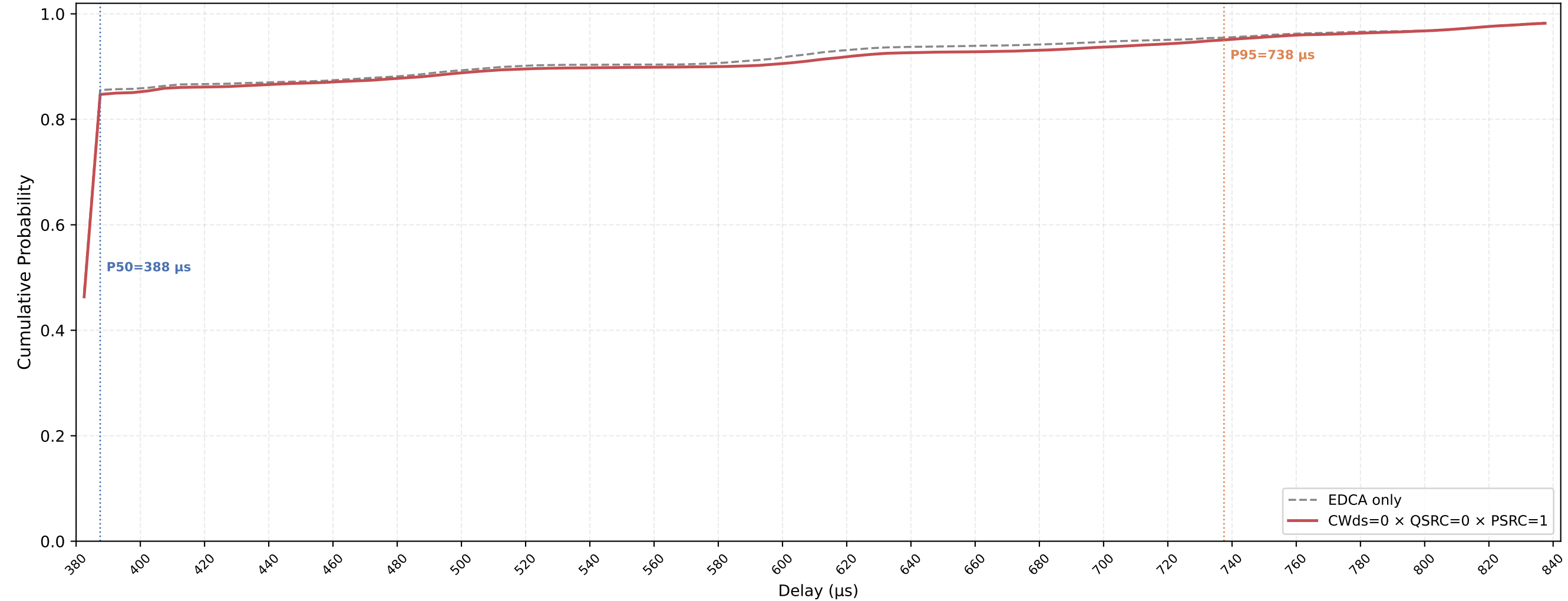
Legacy STA VO Delay CDF — CWds=0 × QSRC=0 × PSRC=1 nSta=30, nPedca=5, 0.1Mbps, avg of 10 runs
