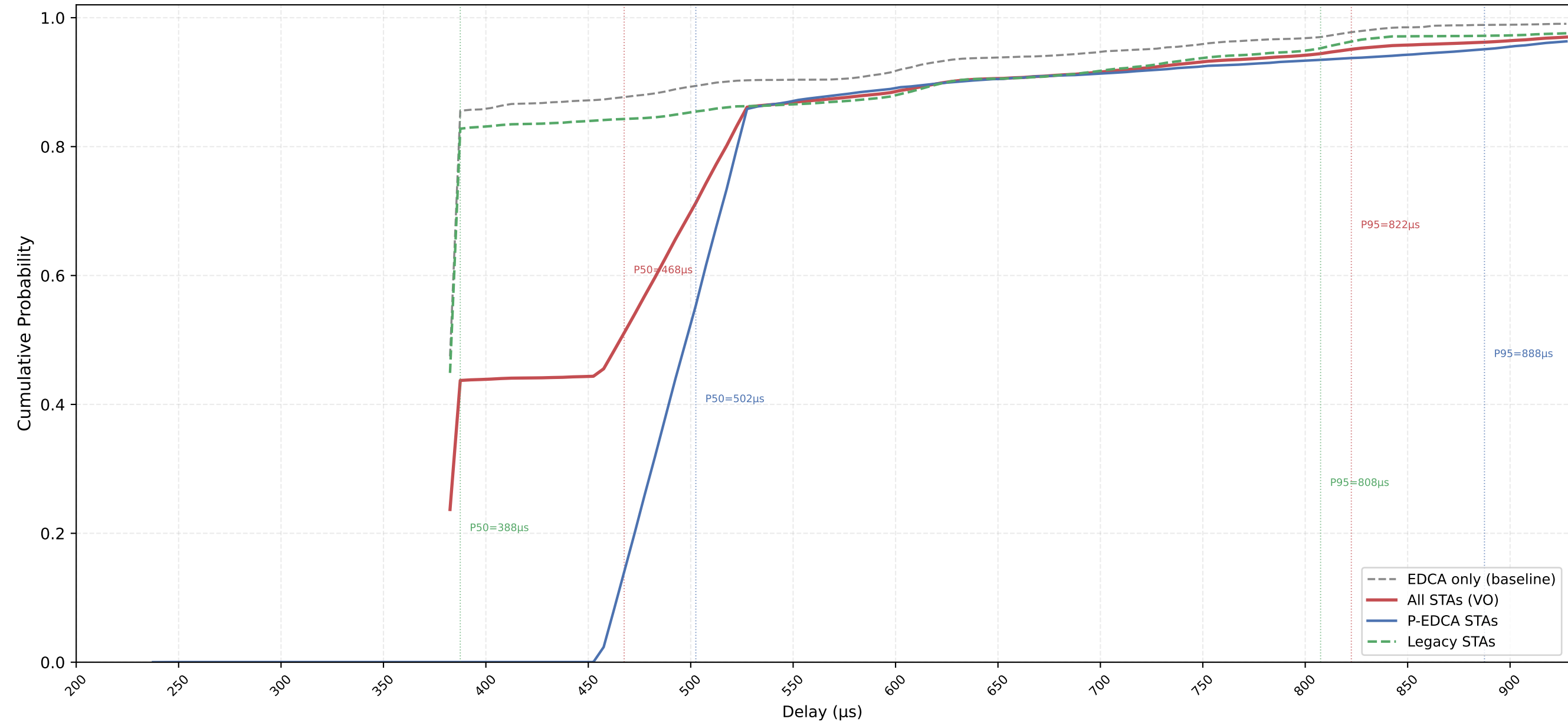
VO Delay CDF — P-EDCA / Legacy / All | CWds=0 × QSRC=0 × PSRC=2 nSta=30, nPedca=15/30, 0.1Mbps, avg of 10 runs
