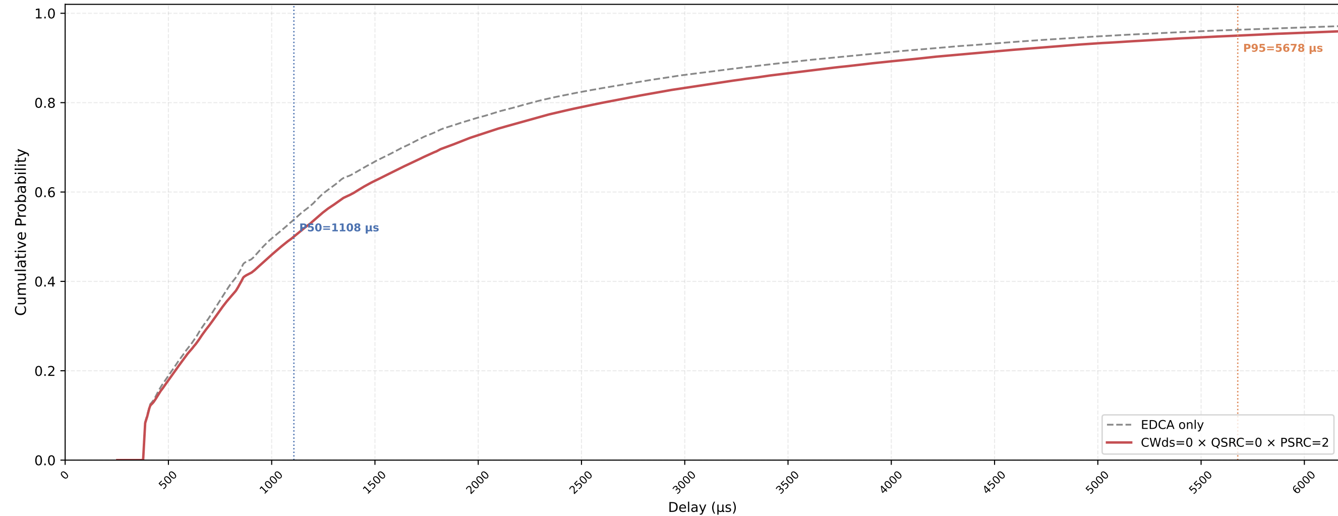
Legacy STA VO Delay CDF — CWds=0 × QSRC=0 × PSRC=2 nSta=30, nPedca=5, 0.5Mbps, avg of 10 runs
